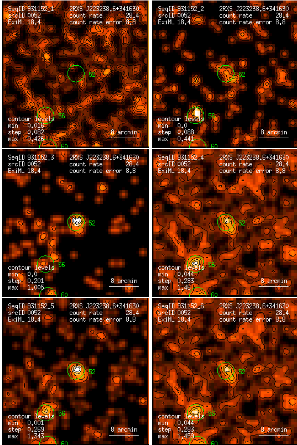
Figure 52: RASS 931152: detection 0052: band rate images, Gaussian filter: (1) PSPC channels 11 – 41, (2) 52 – 90, (3) 91 – 201, (4) 11 – 235, (5) 52 – 201, (6) 11 – 201. Broad band rates in counts/ks. Band rate contour levels in counts/ks/arcmin 2 .
