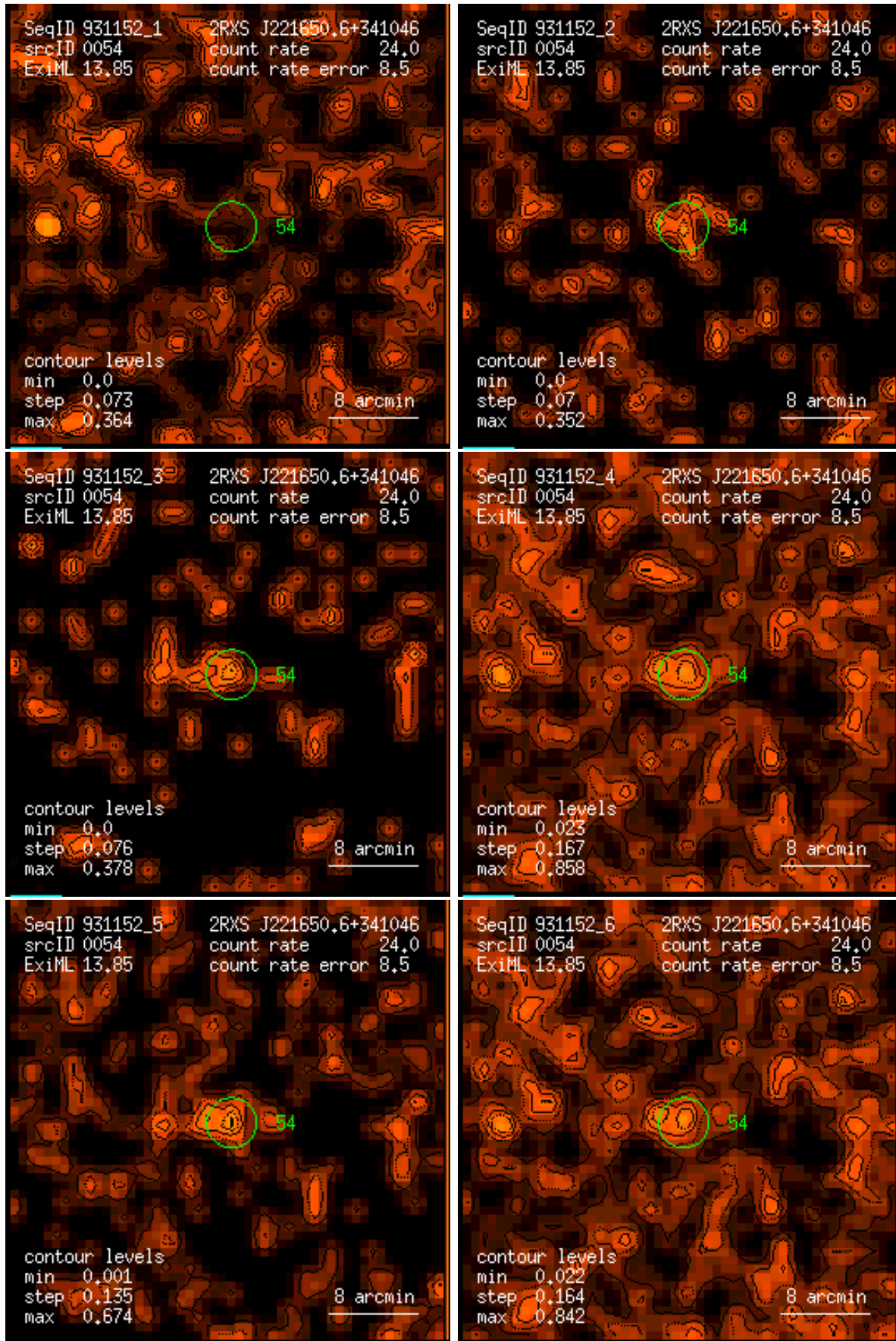
Figure 54: RASS 931152: detection 0054: band rate images, Gaussian filter: (1) PSPC channels 11 – 41, (2) 52 – 90, (3) 91 – 201, (4) 11 – 235, (5) 52 – 201, (6) 11 – 201. Broad band rates in counts/ks. Band rate contour levels in counts/ks/arcmin 2 .
