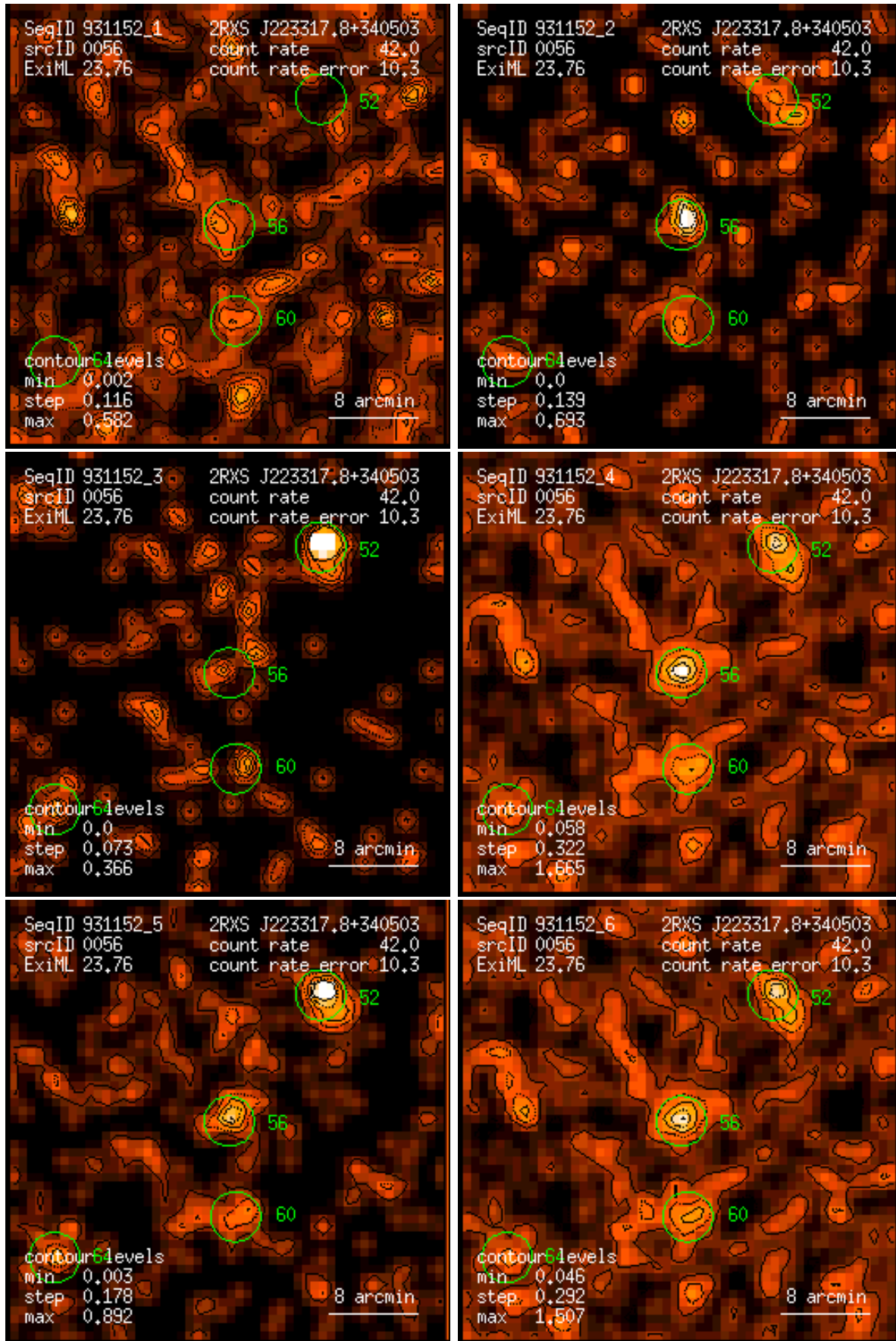
Figure 56: RASS 931152: detection 0056: band rate images, Gaussian filter: (1) PSPC channels 11 – 41, (2) 52 – 90, (3) 91 – 201, (4) 11 – 235, (5) 52 – 201, (6) 11 – 201. Broad band rates in counts/ks. Band rate contour levels in counts/ks/arcmin 2 .
