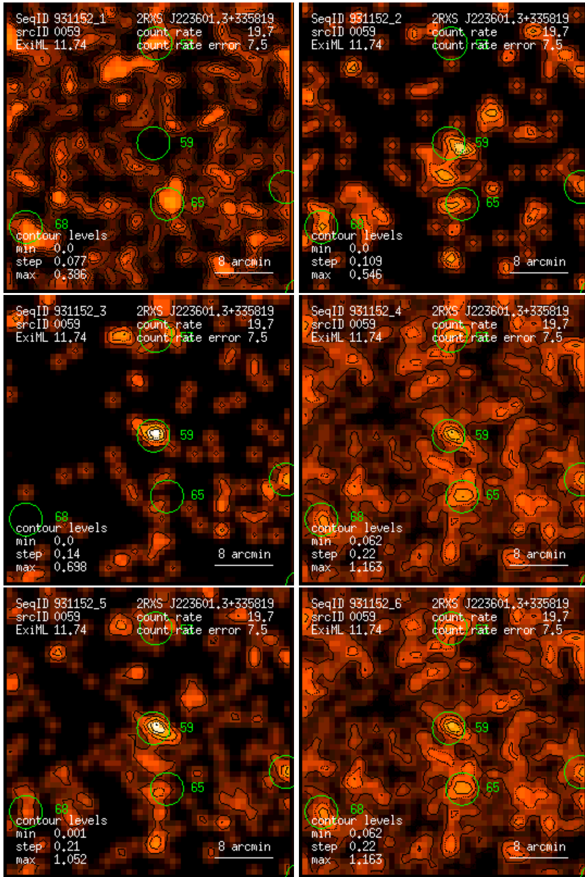
Figure 59: RASS 931152: detection 0059: band rate images, Gaussian filter: (1) PSPC channels 11 – 41, (2) 52 – 90, (3) 91 – 201, (4) 11 – 235, (5) 52 – 201, (6) 11 – 201. Broad band rates in counts/ks. Band rate contour levels in counts/ks/arcmin 2 .
