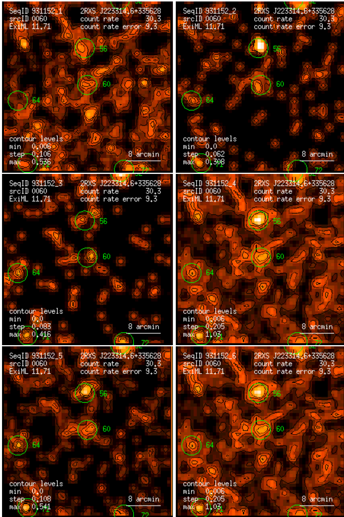
Figure 60: RASS 931152: detection 0060: band rate images, Gaussian filter: (1) PSPC channels 11 – 41, (2) 52 – 90, (3) 91 – 201, (4) 11 – 235, (5) 52 – 201, (6) 11 – 201. Broad band rates in counts/ks. Band rate contour levels in counts/ks/arcmin 2 .
