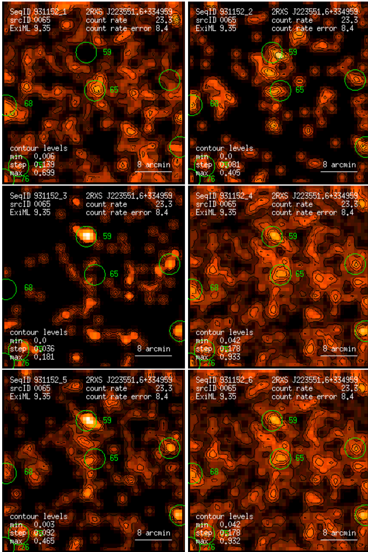
Figure 65: RASS 931152: detection 0065: band rate images, Gaussian filter: (1) PSPC channels 11 – 41, (2) 52 – 90, (3) 91 – 201, (4) 11 – 235, (5) 52 – 201, (6) 11 – 201. Broad band rates in counts/ks. Band rate contour levels in counts/ks/arcmin 2 .
