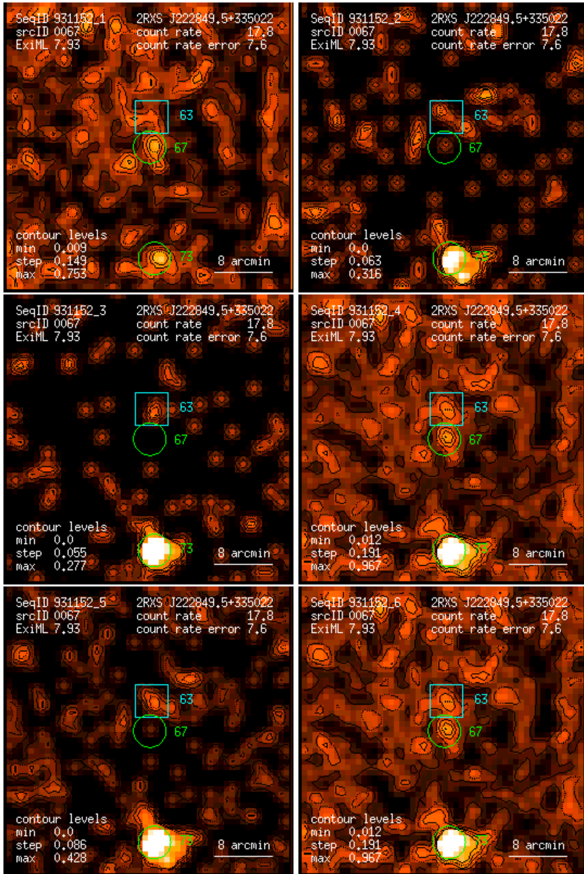
Figure 67: RASS 931152: detection 0067: band rate images, Gaussian filter: (1) PSPC channels 11 – 41, (2) 52 – 90, (3) 91 – 201, (4) 11 – 235, (5) 52 – 201, (6) 11 – 201. Broad band rates in counts/ks. Band rate contour levels in counts/ks/arcmin 2 .
