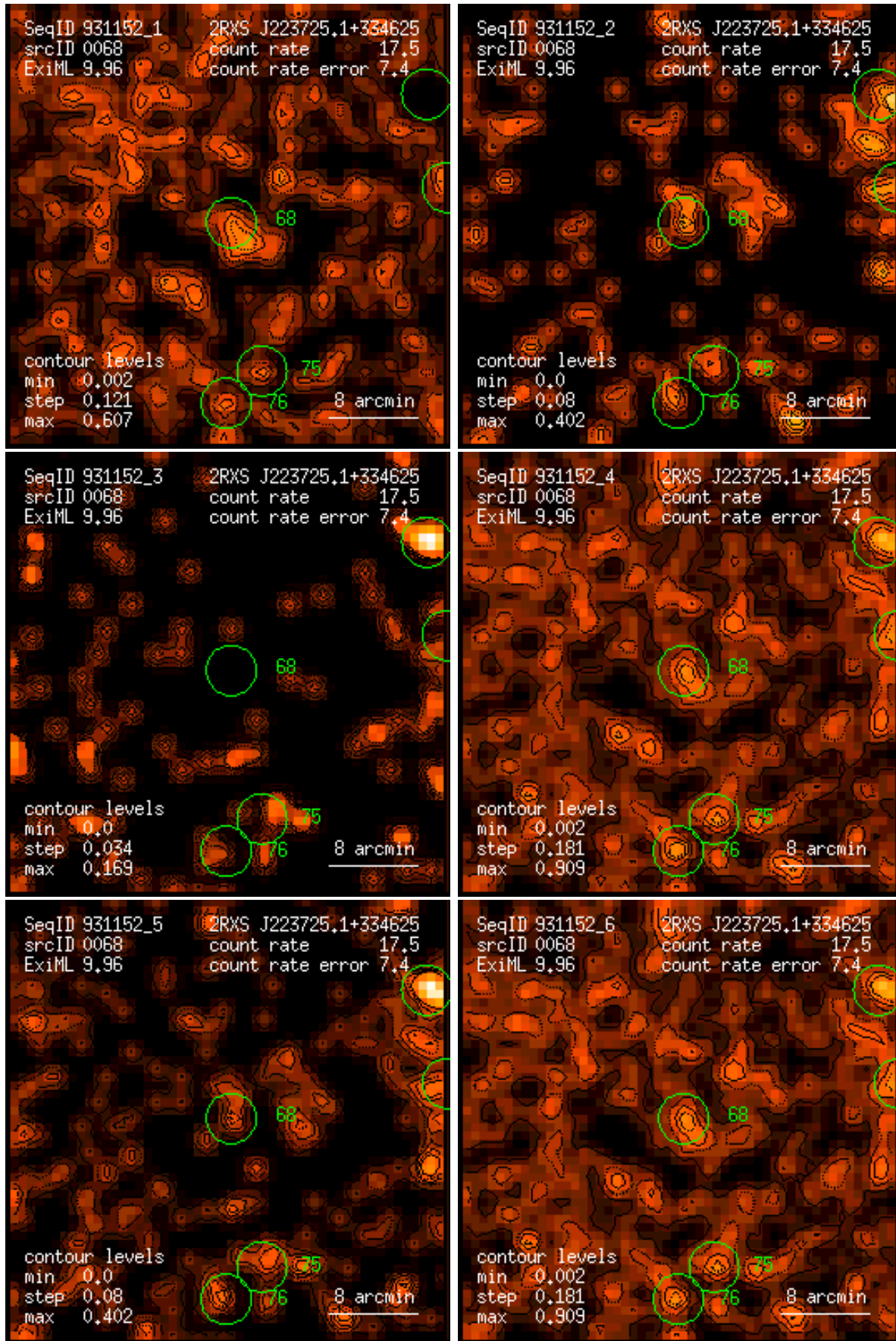
Figure 68: RASS 931152: detection 0068: band rate images, Gaussian filter: (1) PSPC channels 11 – 41, (2) 52 – 90, (3) 91 – 201, (4) 11 – 235, (5) 52 – 201, (6) 11 – 201. Broad band rates in counts/ks. Band rate contour levels in counts/ks/arcmin 2 .
