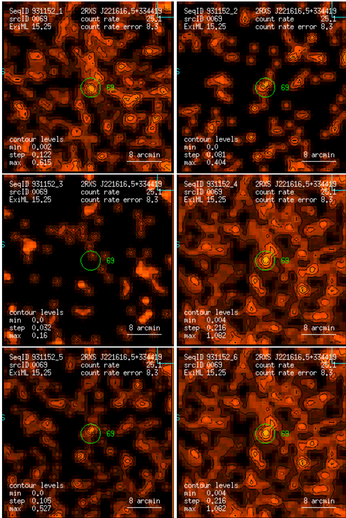
Figure 69: RASS 931152: detection 0069: band rate images, Gaussian filter: (1) PSPC channels 11 – 41, (2) 52 – 90, (3) 91 – 201, (4) 11 – 235, (5) 52 – 201, (6) 11 – 201. Broad band rates in counts/ks. Band rate contour levels in counts/ks/arcmin 2 .
