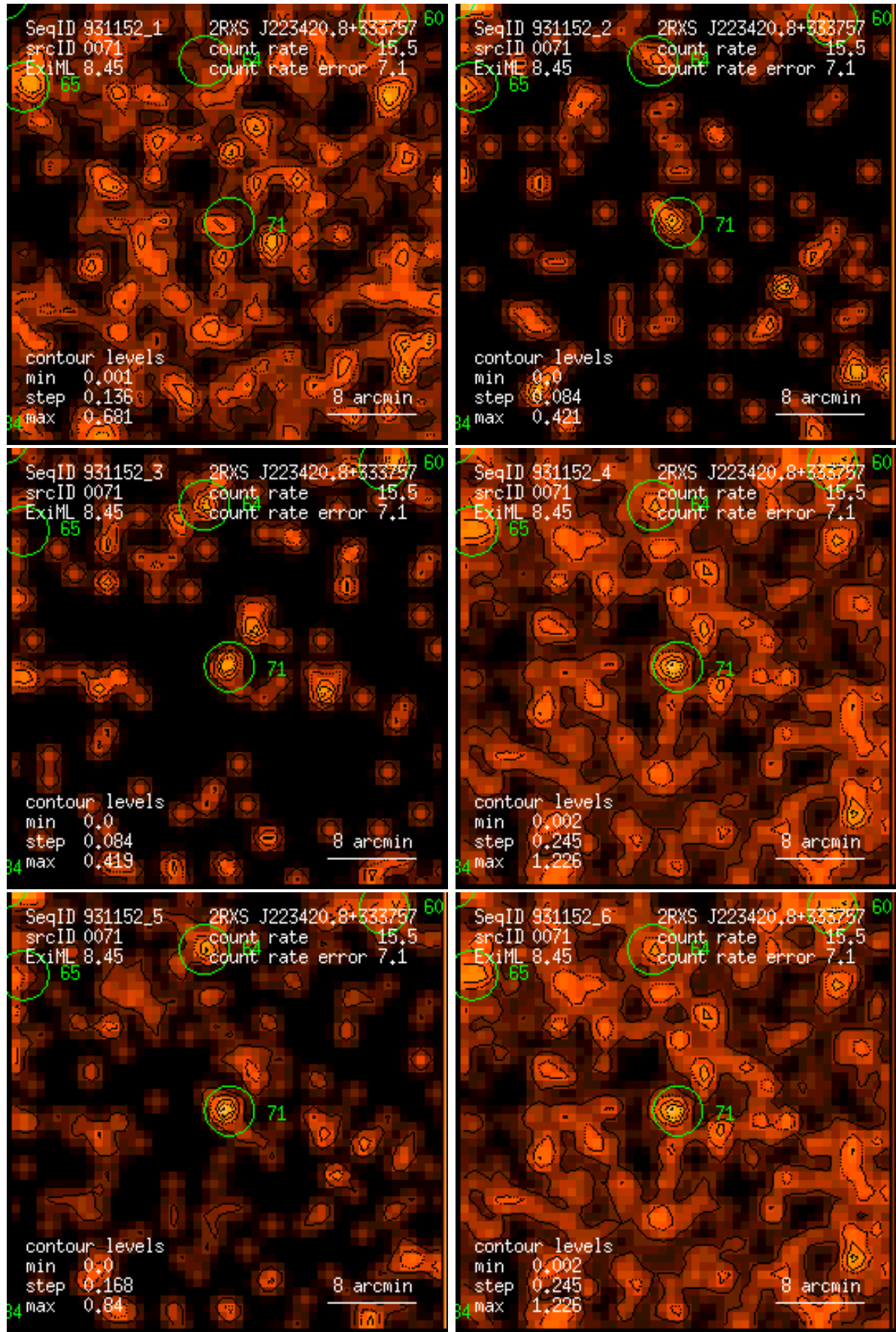
Figure 71: RASS 931152: detection 0071: band rate images, Gaussian filter: (1) PSPC channels 11 – 41, (2) 52 – 90, (3) 91 – 201, (4) 11 – 235, (5) 52 – 201, (6) 11 – 201. Broad band rates in counts/ks. Band rate contour levels in counts/ks/arcmin 2 .
