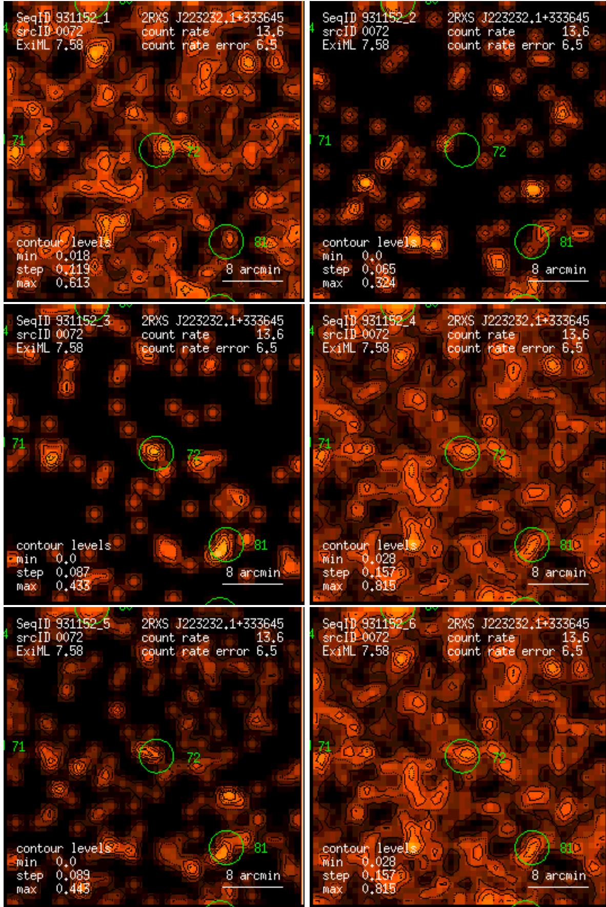
Figure 72: RASS 931152: detection 0072: band rate images, Gaussian filter: (1) PSPC channels 11 – 41, (2) 52 – 90, (3) 91 – 201, (4) 11 – 235, (5) 52 – 201, (6) 11 – 201. Broad band rates in counts/ks. Band rate contour levels in counts/ks/arcmin 2 .
