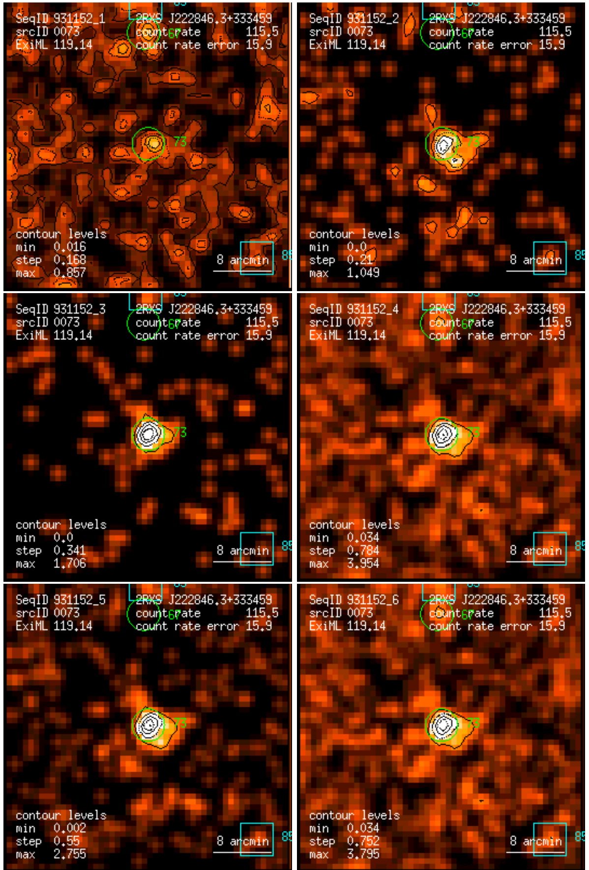
Figure 73: RASS 931152: detection 0073: band rate images, Gaussian filter: (1) PSPC channels 11 – 41, (2) 52 – 90, (3) 91 – 201, (4) 11 – 235, (5) 52 – 201, (6) 11 – 201. Broad band rates in counts/ks. Band rate contour levels in counts/ks/arcmin 2 .
