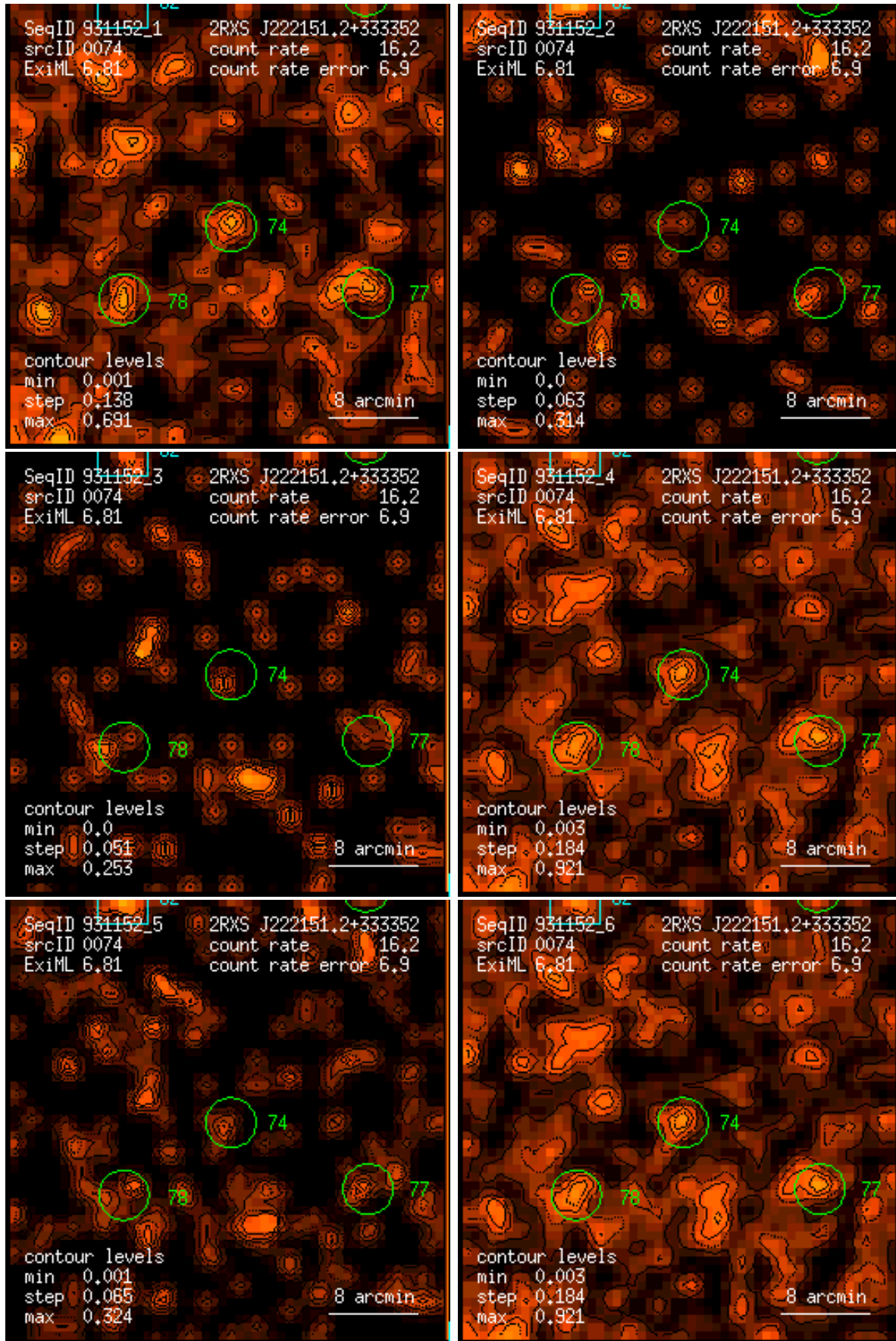
Figure 74: RASS 931152: detection 0074: band rate images, Gaussian filter: (1) PSPC channels 11 – 41, (2) 52 – 90, (3) 91 – 201, (4) 11 – 235, (5) 52 – 201, (6) 11 – 201. Broad band rates in counts/ks. Band rate contour levels in counts/ks/arcmin 2 .
