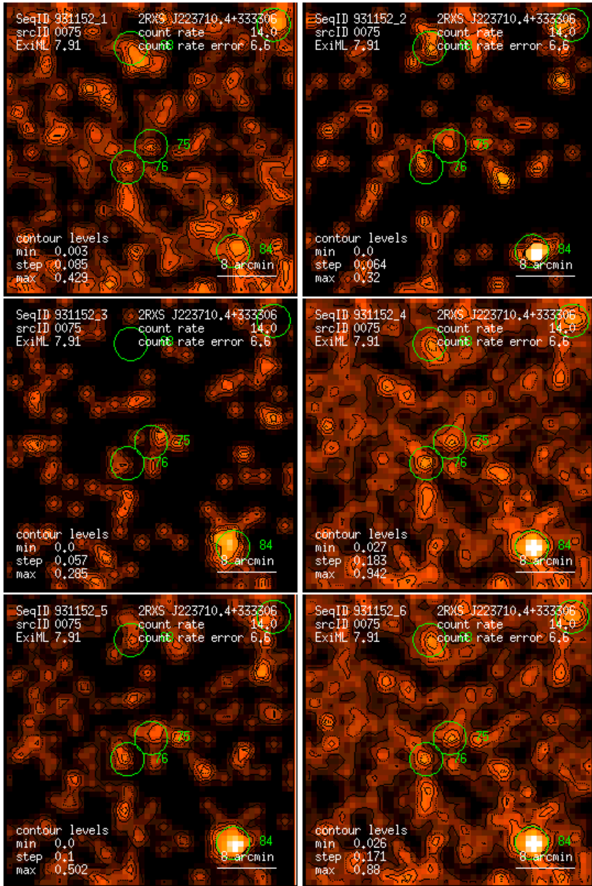
Figure 75: RASS 931152: detection 0075: band rate images, Gaussian filter: (1) PSPC channels 11 – 41, (2) 52 – 90, (3) 91 – 201, (4) 11 – 235, (5) 52 – 201, (6) 11 – 201. Broad band rates in counts/ks. Band rate contour levels in counts/ks/arcmin 2 .
