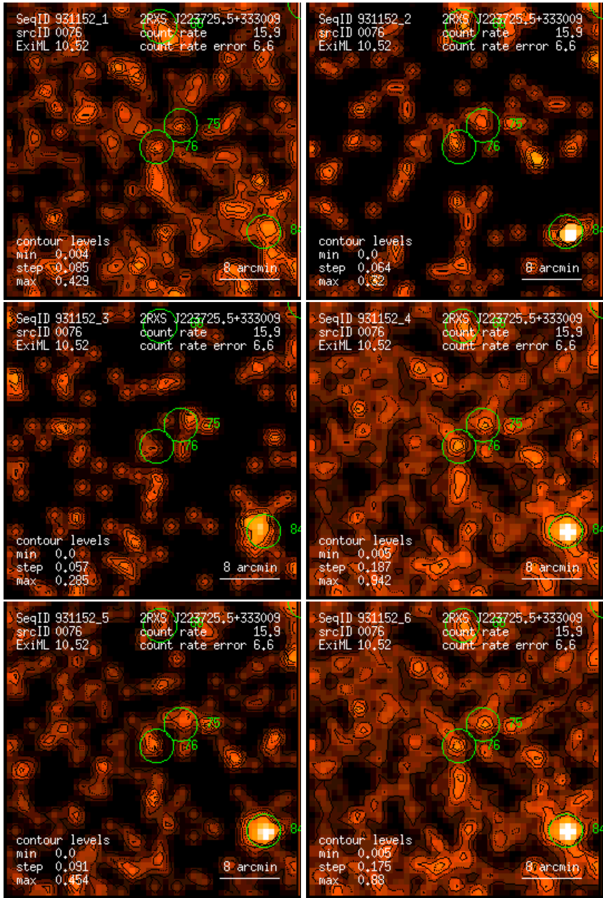
Figure 76: RASS 931152: detection 0076: band rate images, Gaussian filter: (1) PSPC channels 11 – 41, (2) 52 – 90, (3) 91 – 201, (4) 11 – 235, (5) 52 – 201, (6) 11 – 201. Broad band rates in counts/ks. Band rate contour levels in counts/ks/arcmin 2 .
