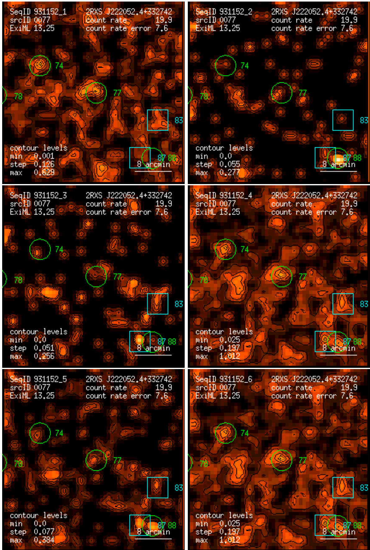
Figure 77: RASS 931152: detection 0077: band rate images, Gaussian filter: (1) PSPC channels 11 – 41, (2) 52 – 90, (3) 91 – 201, (4) 11 – 235, (5) 52 – 201, (6) 11 – 201. Broad band rates in counts/ks. Band rate contour levels in counts/ks/arcmin 2 .
