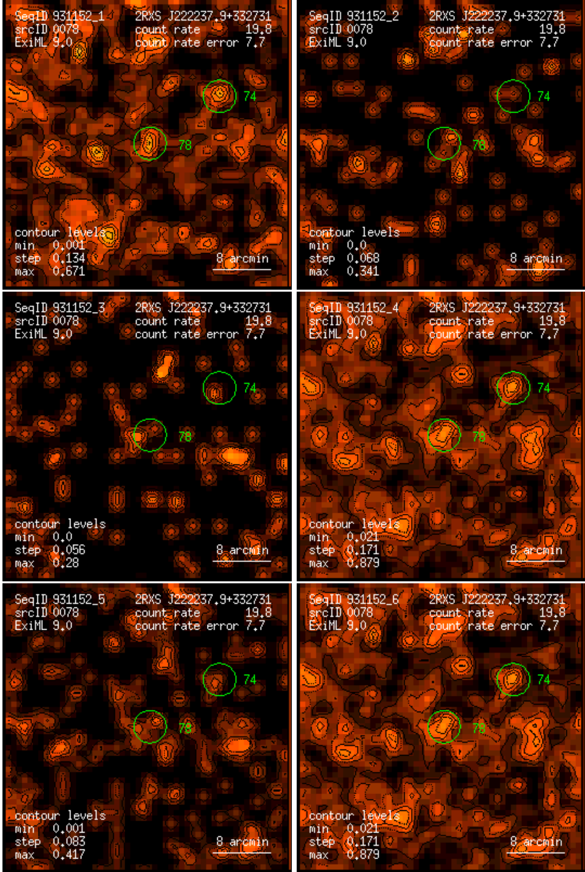
Figure 78: RASS 931152: detection 0078: band rate images, Gaussian filter: (1) PSPC channels 11 – 41, (2) 52 – 90, (3) 91 – 201, (4) 11 – 235, (5) 52 – 201, (6) 11 – 201. Broad band rates in counts/ks. Band rate contour levels in counts/ks/arcmin 2 .
