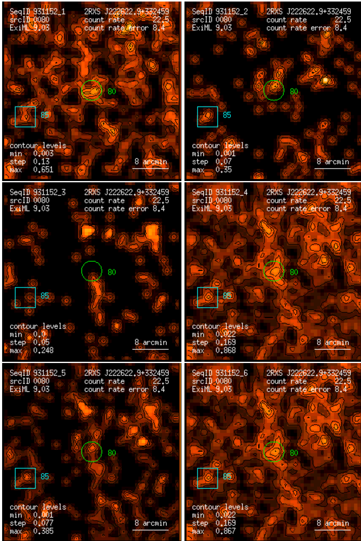
Figure 80: RASS 931152: detection 0080: band rate images, Gaussian filter: (1) PSPC channels 11 – 41, (2) 52 – 90, (3) 91 – 201, (4) 11 – 235, (5) 52 – 201, (6) 11 – 201. Broad band rates in counts/ks. Band rate contour levels in counts/ks/arcmin 2 .
