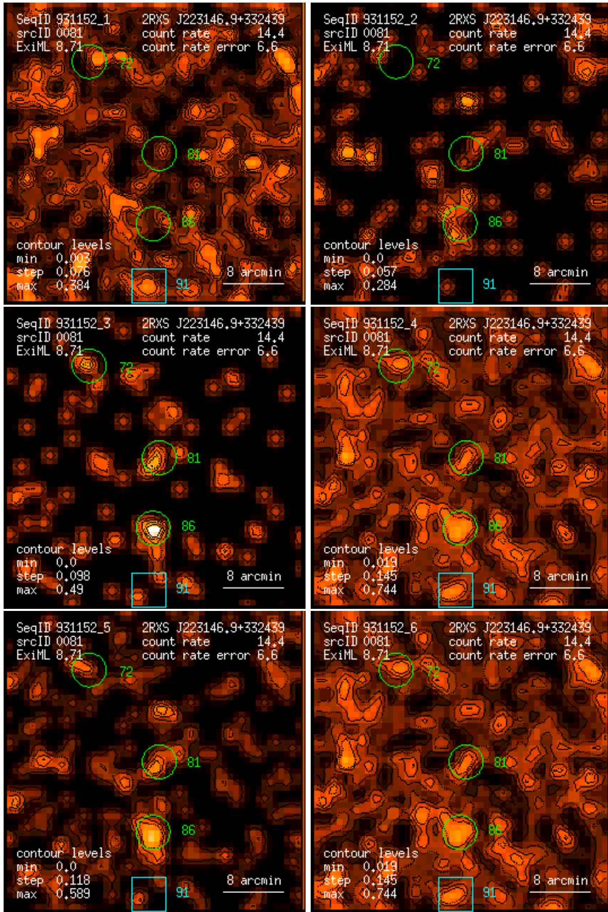
Figure 81: RASS 931152: detection 0081: band rate images, Gaussian filter: (1) PSPC channels 11 – 41, (2) 52 – 90, (3) 91 – 201, (4) 11 – 235, (5) 52 – 201, (6) 11 – 201. Broad band rates in counts/ks. Band rate contour levels in counts/ks/arcmin 2 .
