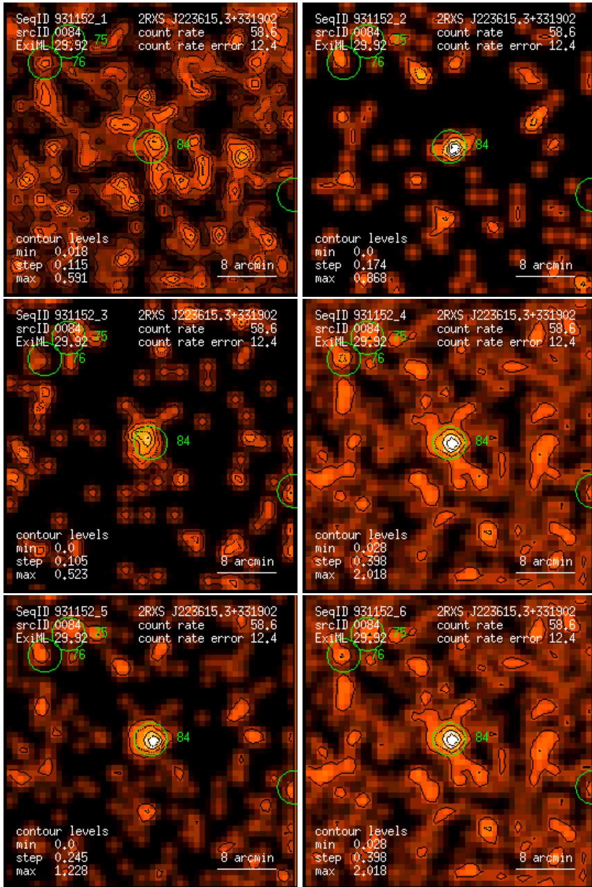
Figure 84: RASS 931152: detection 0084: band rate images, Gaussian filter: (1) PSPC channels 11 – 41, (2) 52 – 90, (3) 91 – 201, (4) 11 – 235, (5) 52 – 201, (6) 11 – 201. Broad band rates in counts/ks. Band rate contour levels in counts/ks/arcmin 2 .
