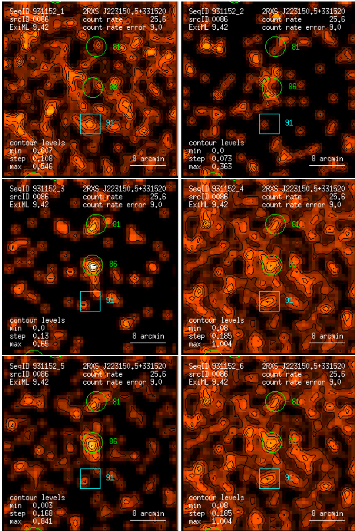
Figure 86: RASS 931152: detection 0086: band rate images, Gaussian filter: (1) PSPC channels 11 – 41, (2) 52 – 90, (3) 91 – 201, (4) 11 – 235, (5) 52 – 201, (6) 11 – 201. Broad band rates in counts/ks. Band rate contour levels in counts/ks/arcmin 2 .
