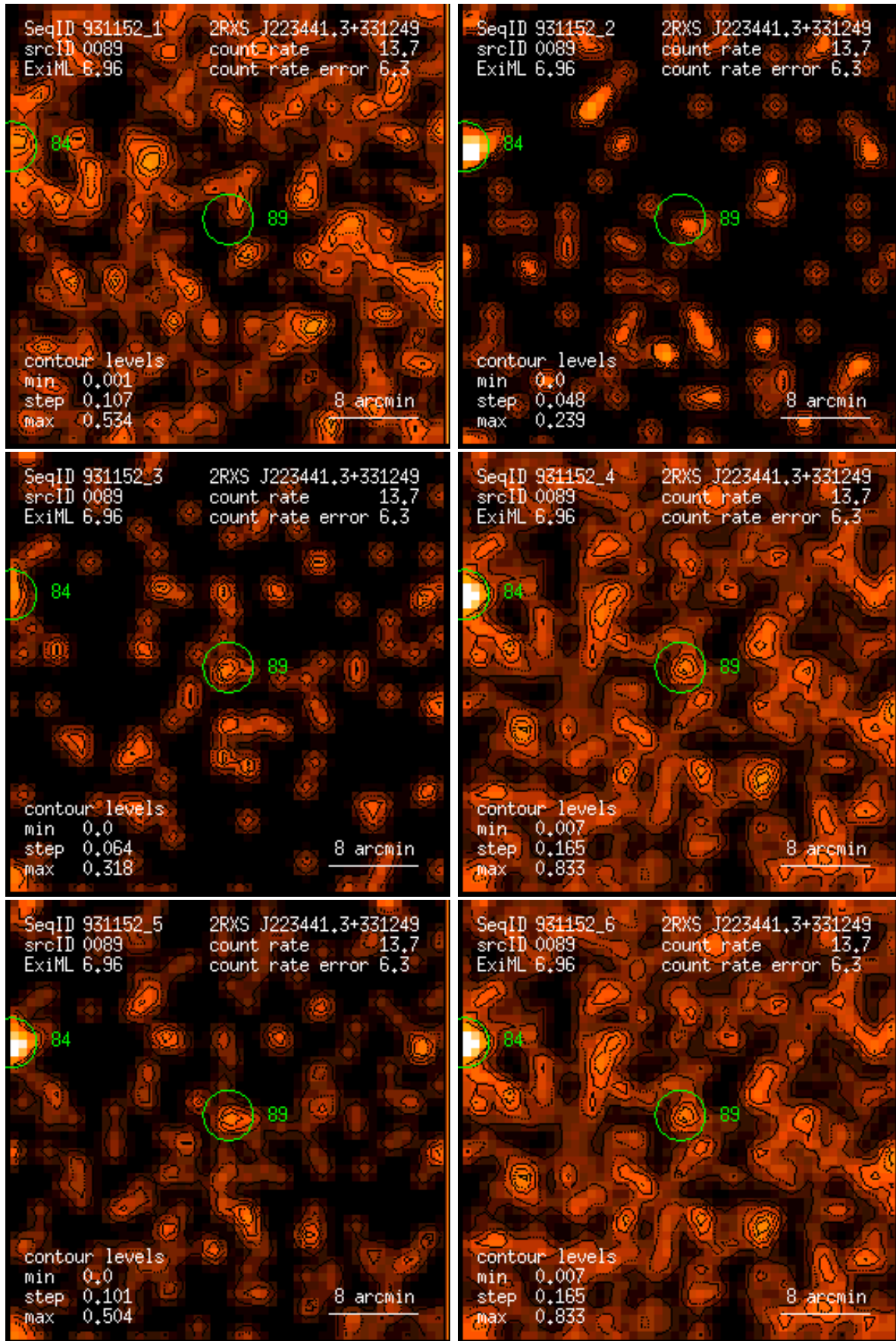
Figure 89: RASS 931152: detection 0089: band rate images, Gaussian filter: (1) PSPC channels 11 – 41, (2) 52 – 90, (3) 91 – 201, (4) 11 – 235, (5) 52 – 201, (6) 11 – 201. Broad band rates in counts/ks. Band rate contour levels in counts/ks/arcmin 2 .
