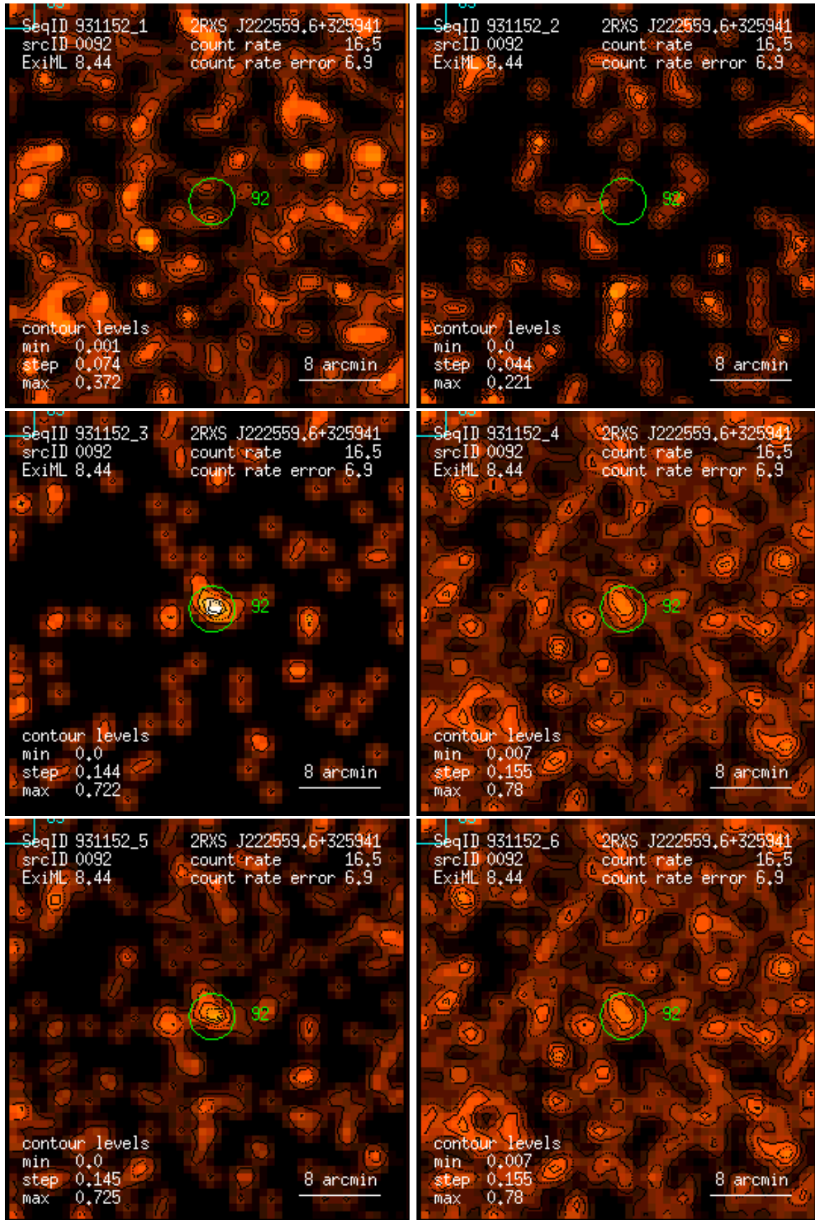
Figure 92: RASS 931152: detection 0092: band rate images, Gaussian filter: (1) PSPC channels 11 – 41, (2) 52 – 90, (3) 91 – 201, (4) 11 – 235, (5) 52 – 201, (6) 11 – 201. Broad band rates in counts/ks. Band rate contour levels in counts/ks/arcmin 2 .
