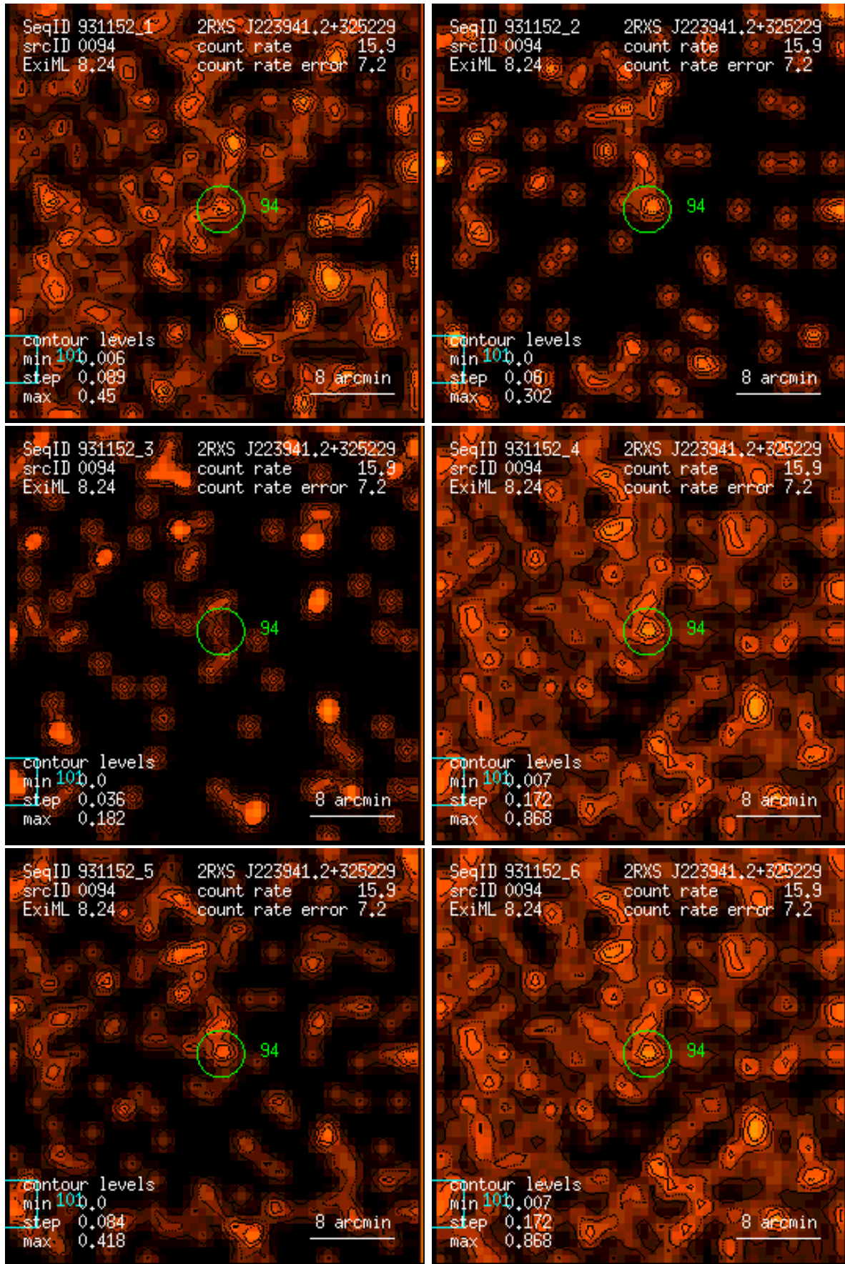
Figure 94: RASS 931152: detection 0094: band rate images, Gaussian filter: (1) PSPC channels 11 – 41, (2) 52 – 90, (3) 91 – 201, (4) 11 – 235, (5) 52 – 201, (6) 11 – 201. Broad band rates in counts/ks. Band rate contour levels in counts/ks/arcmin 2 .
