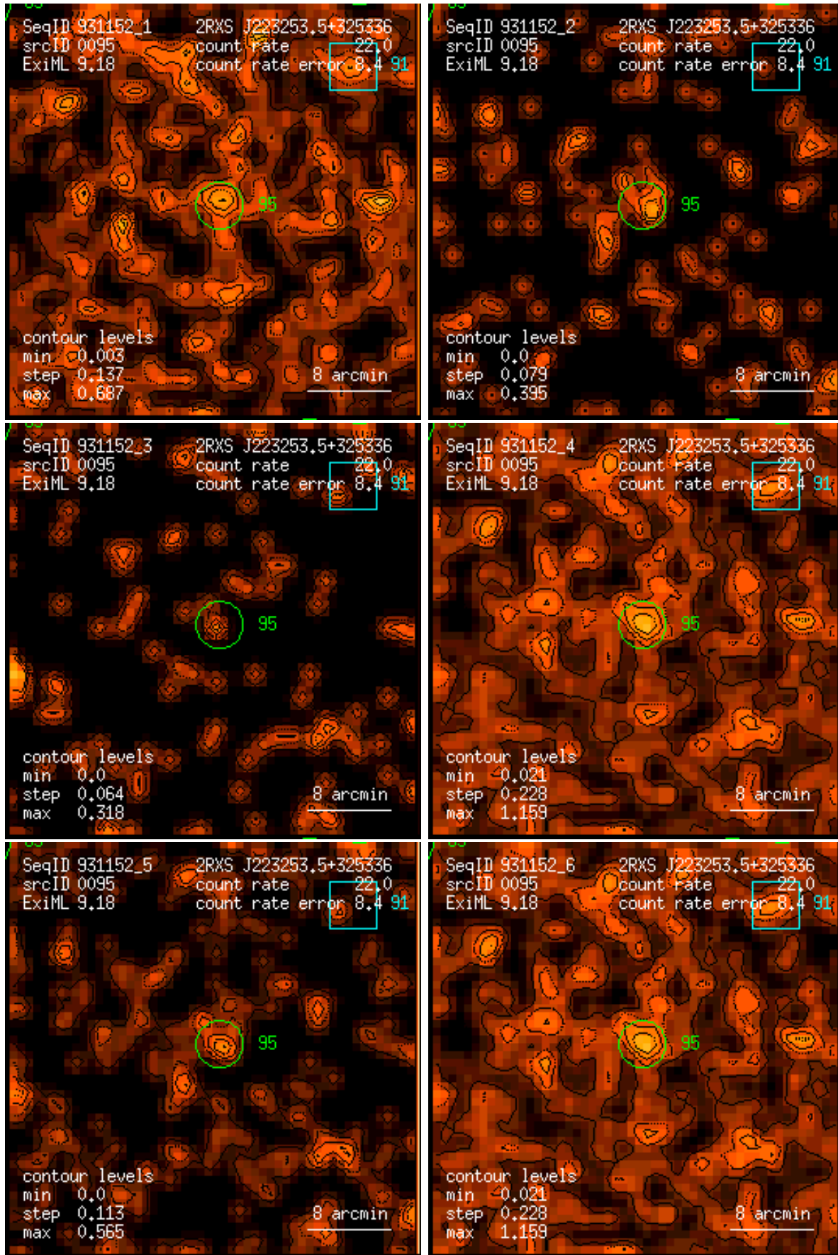
Figure 95: RASS 931152: detection 0095: band rate images, Gaussian filter: (1) PSPC channels 11 – 41, (2) 52 – 90, (3) 91 – 201, (4) 11 – 235, (5) 52 – 201, (6) 11 – 201. Broad band rates in counts/ks. Band rate contour levels in counts/ks/arcmin 2 .
