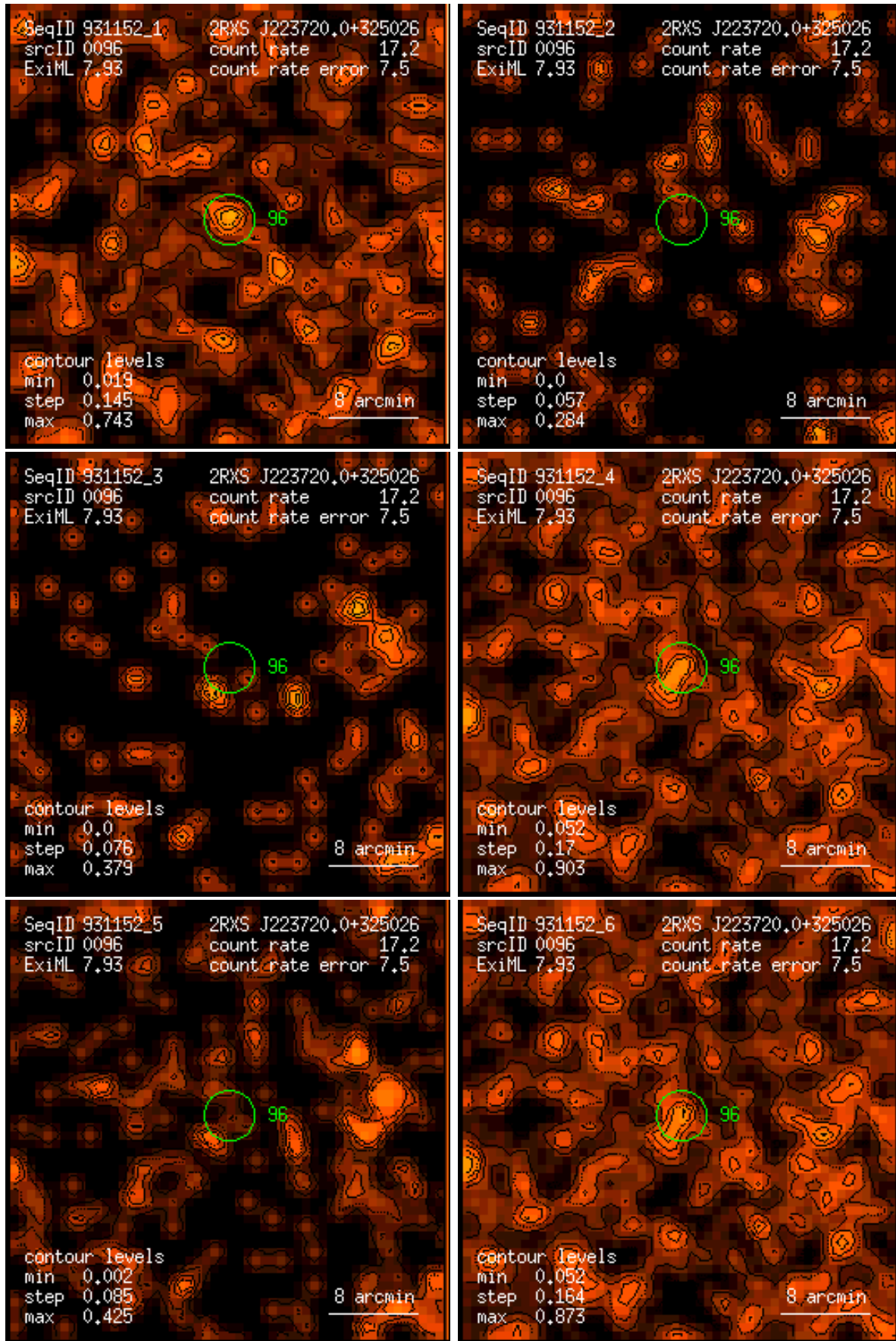
Figure 96: RASS 931152: detection 0096: band rate images, Gaussian filter: (1) PSPC channels 11 – 41, (2) 52 – 90, (3) 91 – 201, (4) 11 – 235, (5) 52 – 201, (6) 11 – 201. Broad band rates in counts/ks. Band rate contour levels in counts/ks/arcmin 2 .
