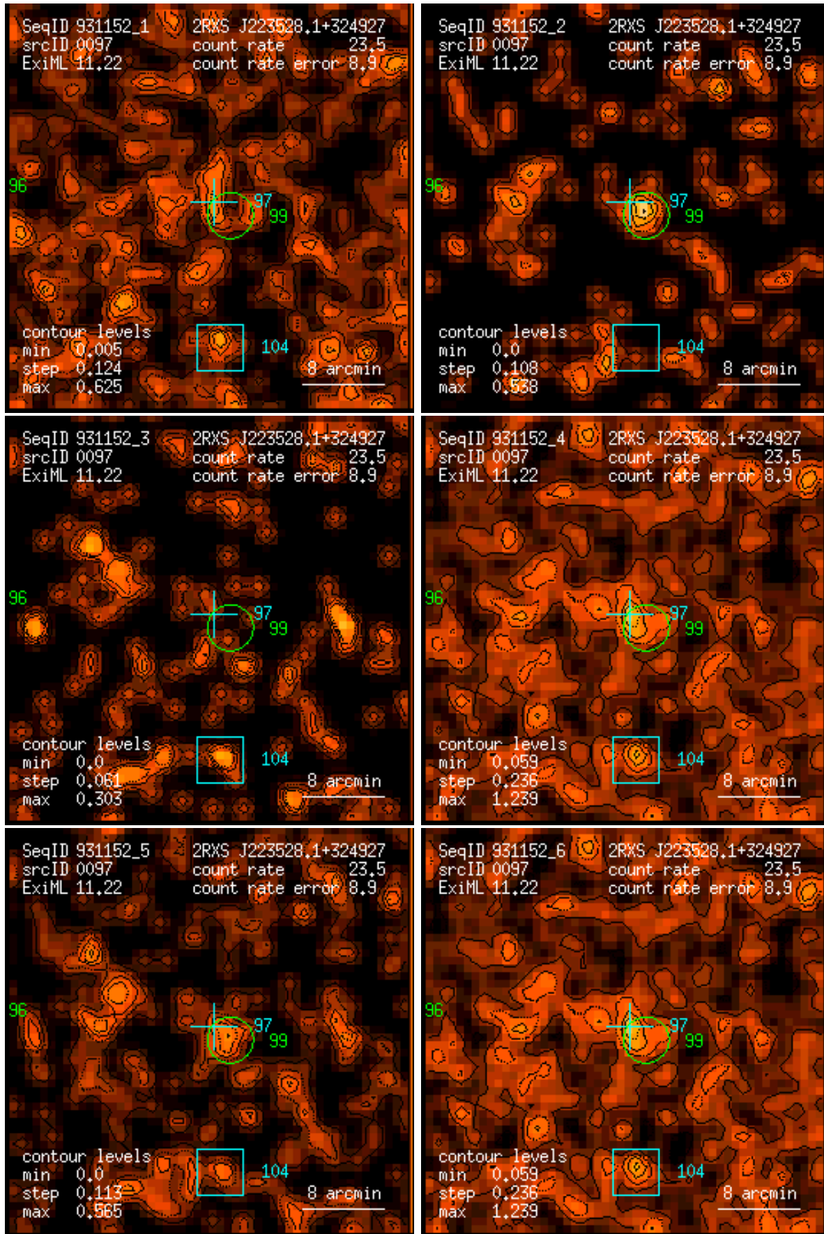
Figure 97: RASS 931152: detection 0097: band rate images, Gaussian filter: (1) PSPC channels 11 – 41, (2) 52 – 90, (3) 91 – 201, (4) 11 – 235, (5) 52 – 201, (6) 11 – 201. Broad band rates in counts/ks. Band rate contour levels in counts/ks/arcmin 2 .
