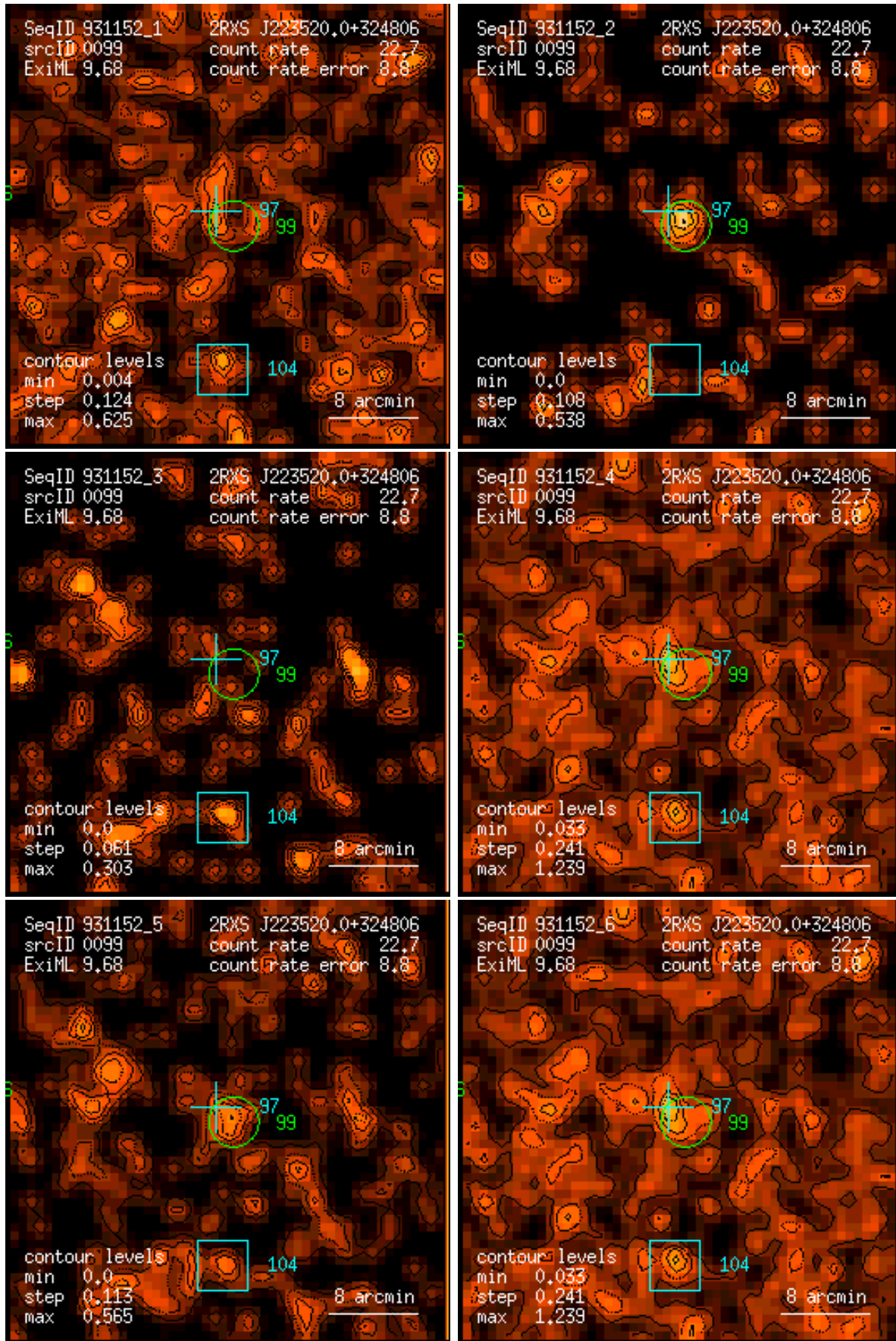
Figure 99: RASS 931152: detection 0099: band rate images, Gaussian filter: (1) PSPC channels 11 – 41, (2) 52 – 90, (3) 91 – 201, (4) 11 – 235, (5) 52 – 201, (6) 11 – 201. Broad band rates in counts/ks. Band rate contour levels in counts/ks/arcmin 2 .
