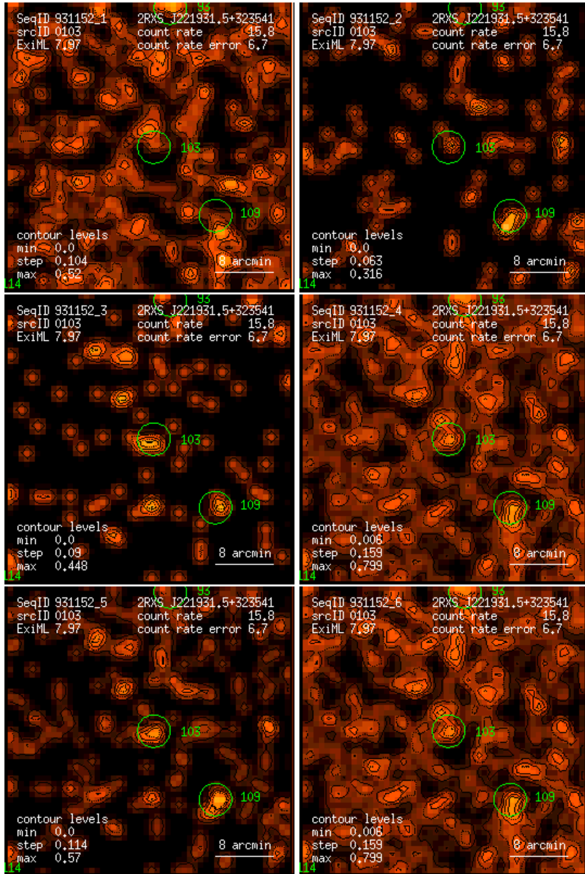
Figure 103: RASS 931152: detection 0103: band rate images, Gaussian filter: (1) PSPC channels 11 – 41, (2) 52 – 90, (3) 91 – 201, (4) 11 – 235, (5) 52 – 201, (6) 11 – 201. Broad band rates in counts/ks. Band rate contour levels in counts/ks/arcmin 2 .
