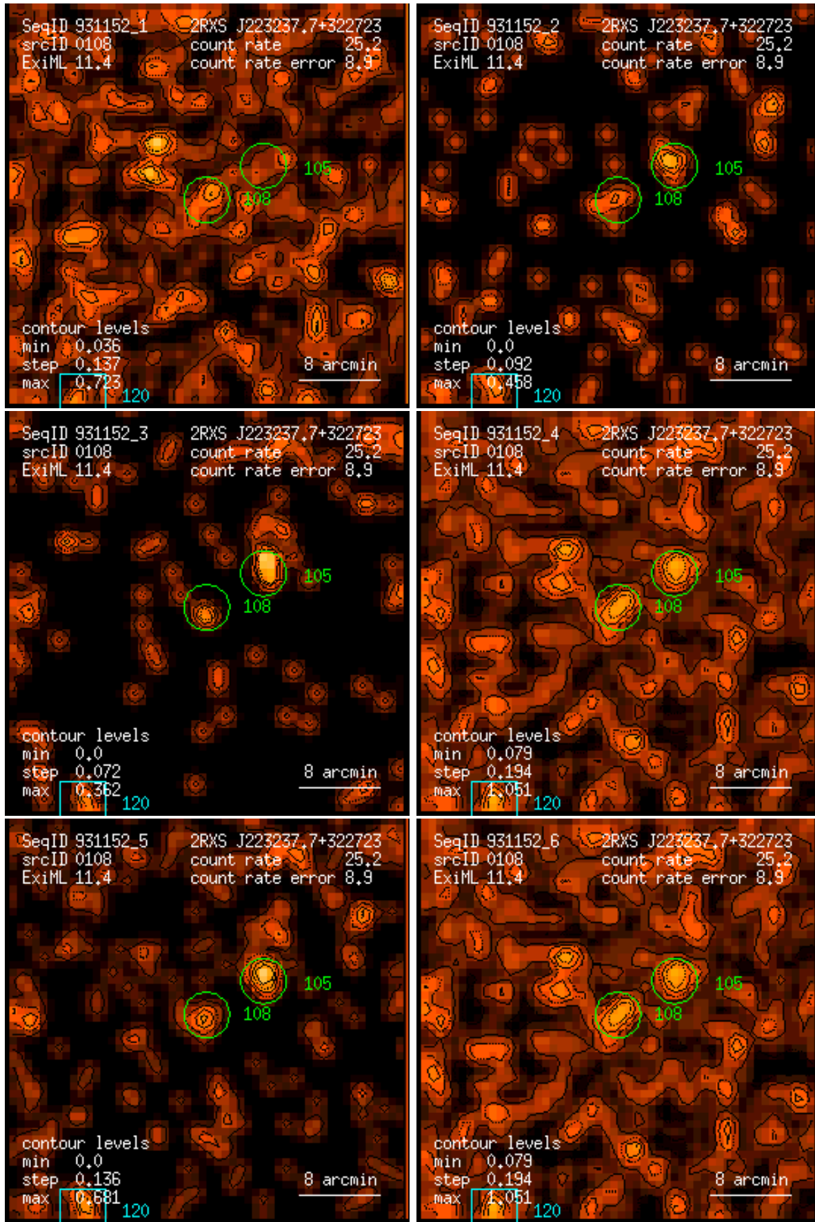
Figure 108: RASS 931152: detection 0108: band rate images, Gaussian filter: (1) PSPC channels 11 – 41, (2) 52 – 90, (3) 91 – 201, (4) 11 – 235, (5) 52 – 201, (6) 11 – 201. Broad band rates in counts/ks. Band rate contour levels in counts/ks/arcmin 2 .
