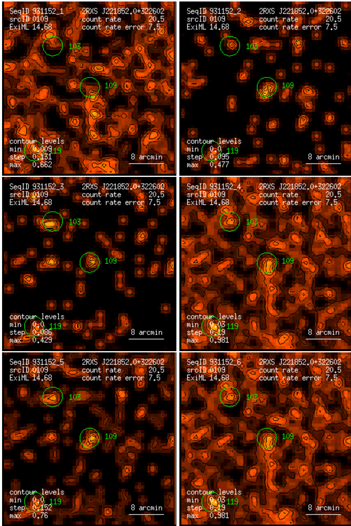
Figure 109: RASS 931152: detection 0109: band rate images, Gaussian filter: (1) PSPC channels 11 – 41, (2) 52 – 90, (3) 91 – 201, (4) 11 – 235, (5) 52 – 201, (6) 11 – 201. Broad band rates in counts/ks. Band rate contour levels in counts/ks/arcmin 2 .
