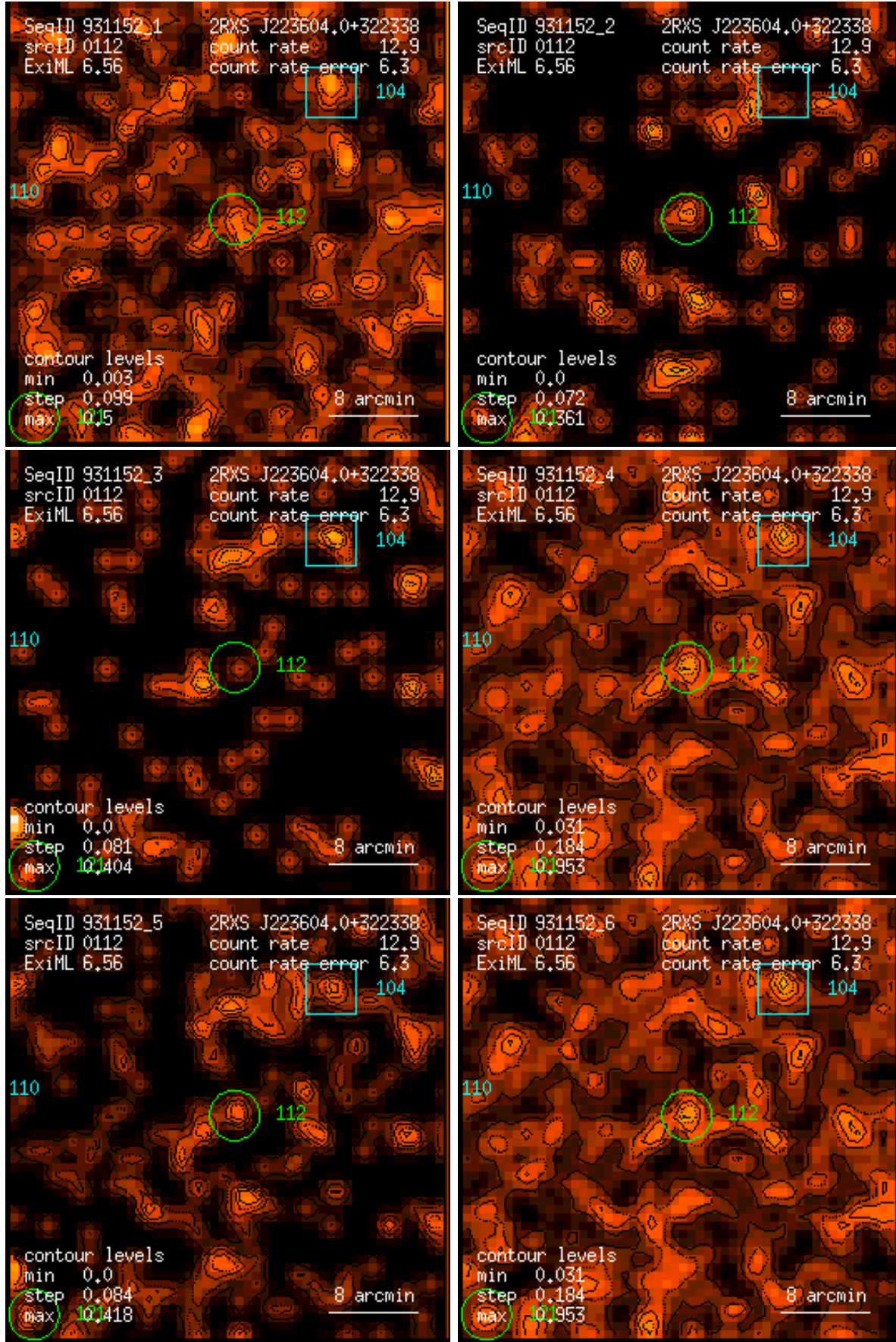
Figure 112: RASS 931152: detection 0112: band rate images, Gaussian filter: (1) PSPC channels 11 – 41, (2) 52 – 90, (3) 91 – 201, (4) 11 – 235, (5) 52 – 201, (6) 11 – 201. Broad band rates in counts/ks. Band rate contour levels in counts/ks/arcmin 2 .
