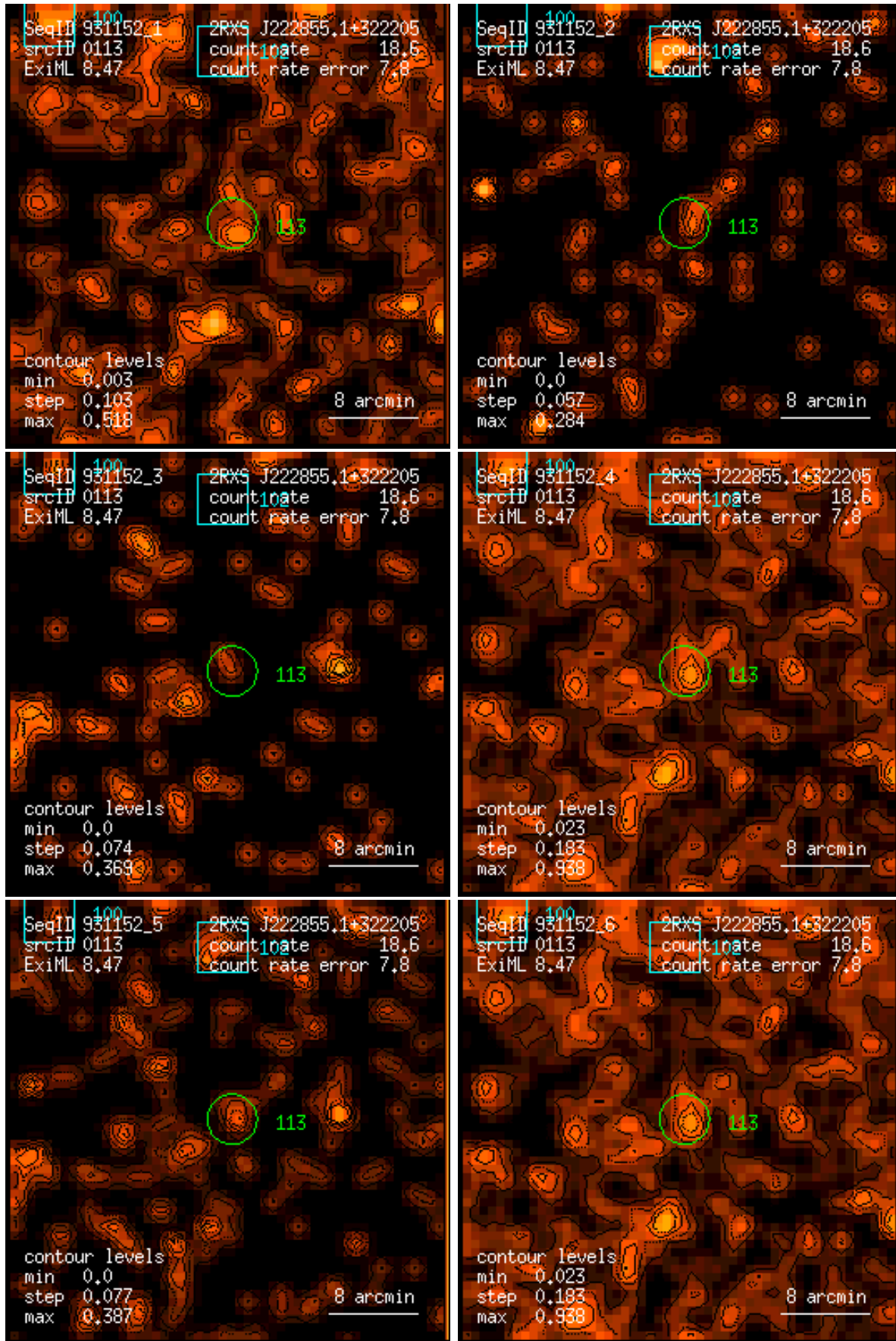
Figure 113: RASS 931152: detection 0113: band rate images, Gaussian filter: (1) PSPC channels 11 – 41, (2) 52 – 90, (3) 91 – 201, (4) 11 – 235, (5) 52 – 201, (6) 11 – 201. Broad band rates in counts/ks. Band rate contour levels in counts/ks/arcmin 2 .
