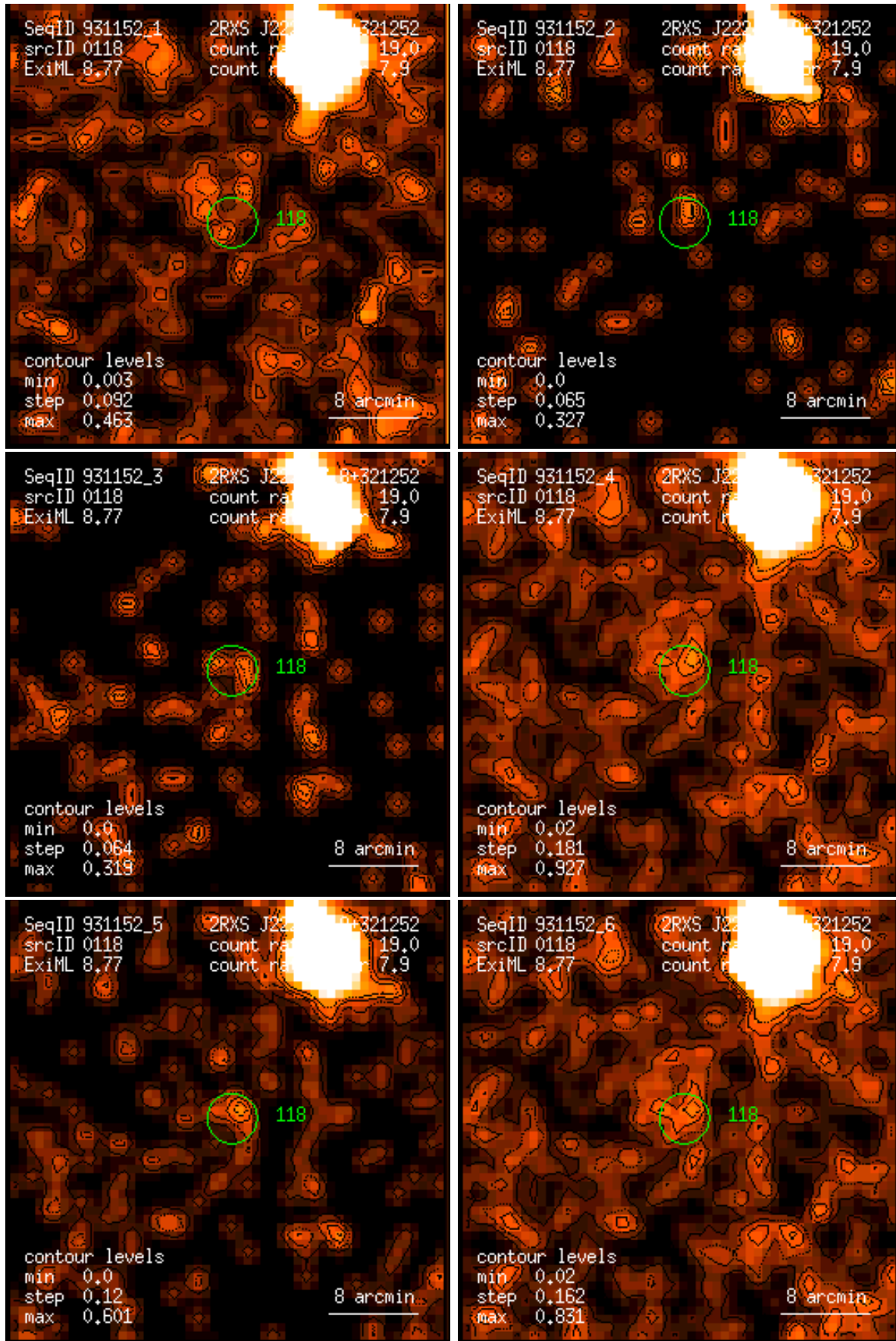
Figure 118: RASS 931152: detection 0118: band rate images, Gaussian filter: (1) PSPC channels 11 – 41, (2) 52 – 90, (3) 91 – 201, (4) 11 – 235, (5) 52 – 201, (6) 11 – 201. Broad band rates in counts/ks. Band rate contour levels in counts/ks/arcmin 2 .
