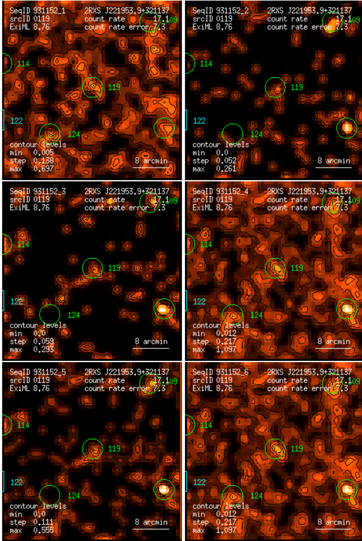
Figure 119: RASS 931152: detection 0119: band rate images, Gaussian filter: (1) PSPC channels 11 – 41, (2) 52 – 90, (3) 91 – 201, (4) 11 – 235, (5) 52 – 201, (6) 11 – 201. Broad band rates in counts/ks. Band rate contour levels in counts/ks/arcmin 2 .
