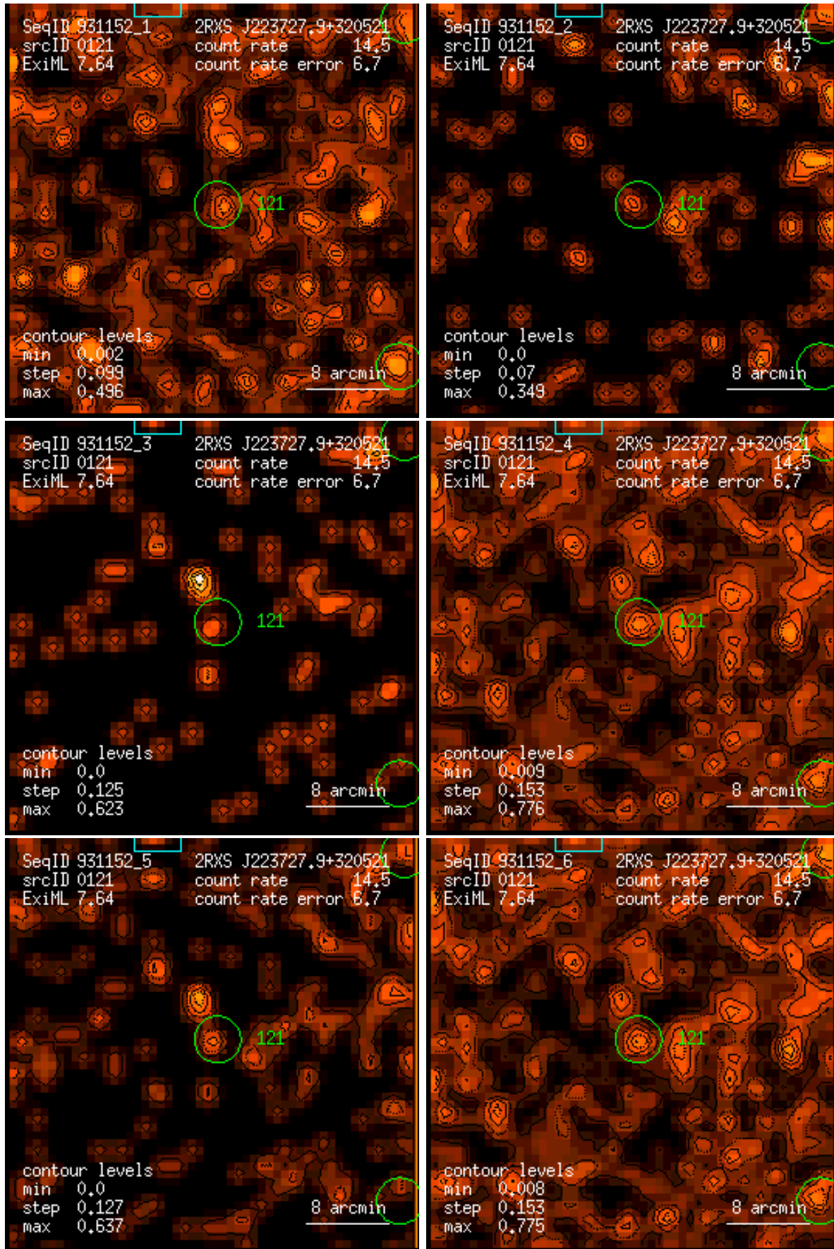
Figure 121: RASS 931152: detection 0121: band rate images, Gaussian filter: (1) PSPC channels 11 – 41, (2) 52 – 90, (3) 91 – 201, (4) 11 – 235, (5) 52 – 201, (6) 11 – 201. Broad band rates in counts/ks. Band rate contour levels in counts/ks/arcmin 2 .
