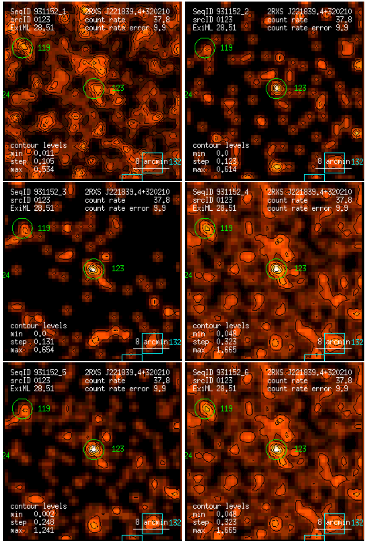
Figure 123: RASS 931152: detection 0123: band rate images, Gaussian filter: (1) PSPC channels 11 – 41, (2) 52 – 90, (3) 91 – 201, (4) 11 – 235, (5) 52 – 201, (6) 11 – 201. Broad band rates in counts/ks. Band rate contour levels in counts/ks/arcmin 2 .
