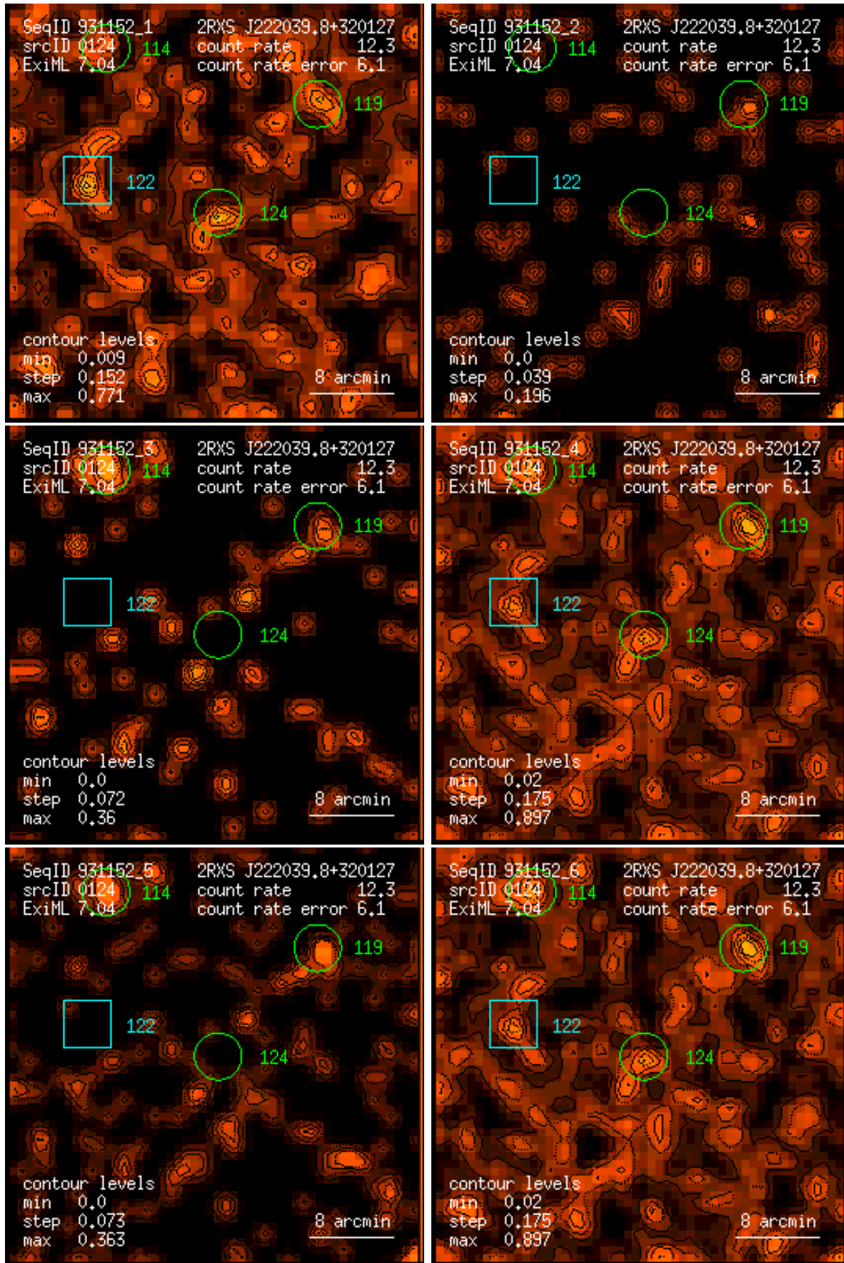
Figure 124: RASS 931152: detection 0124: band rate images, Gaussian filter: (1) PSPC channels 11 – 41, (2) 52 – 90, (3) 91 – 201, (4) 11 – 235, (5) 52 – 201, (6) 11 – 201. Broad band rates in counts/ks. Band rate contour levels in counts/ks/arcmin 2 .
