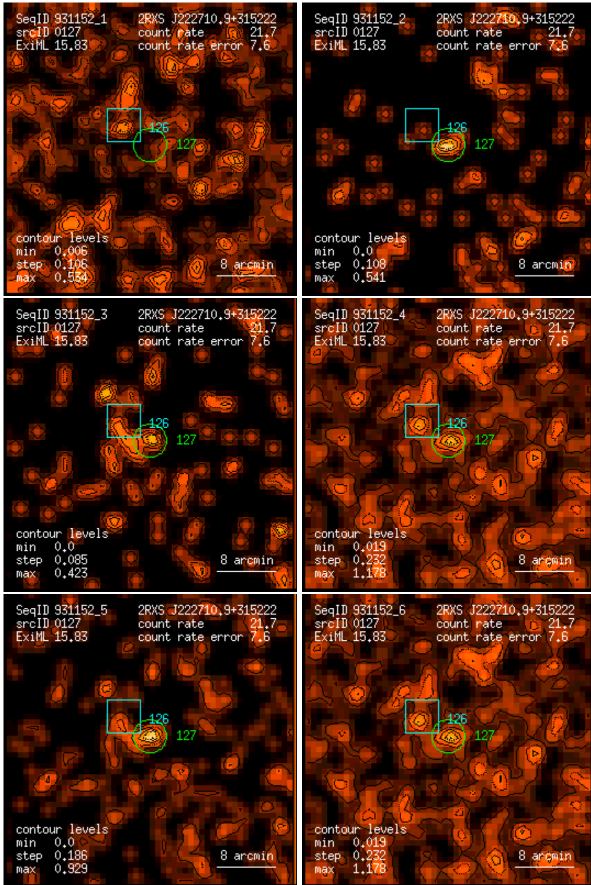
Figure 127: RASS 931152: detection 0127: band rate images, Gaussian filter: (1) PSPC channels 11 – 41, (2) 52 – 90, (3) 91 – 201, (4) 11 – 235, (5) 52 – 201, (6) 11 – 201. Broad band rates in counts/ks. Band rate contour levels in counts/ks/arcmin 2 .
