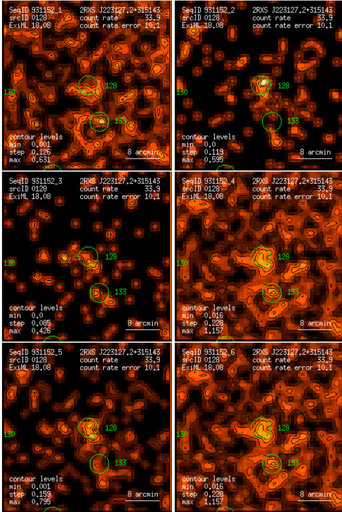
Figure 128: RASS 931152: detection 0128: band rate images, Gaussian filter: (1) PSPC channels 11 – 41, (2) 52 – 90, (3) 91 – 201, (4) 11 – 235, (5) 52 – 201, (6) 11 – 201. Broad band rates in counts/ks. Band rate contour levels in counts/ks/arcmin 2 .
