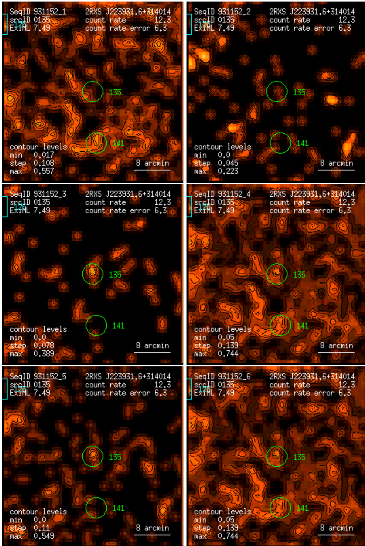
Figure 135: RASS 931152: detection 0135: band rate images, Gaussian filter: (1) PSPC channels 11 – 41, (2) 52 – 90, (3) 91 – 201, (4) 11 – 235, (5) 52 – 201, (6) 11 – 201. Broad band rates in counts/ks. Band rate contour levels in counts/ks/arcmin 2 .
