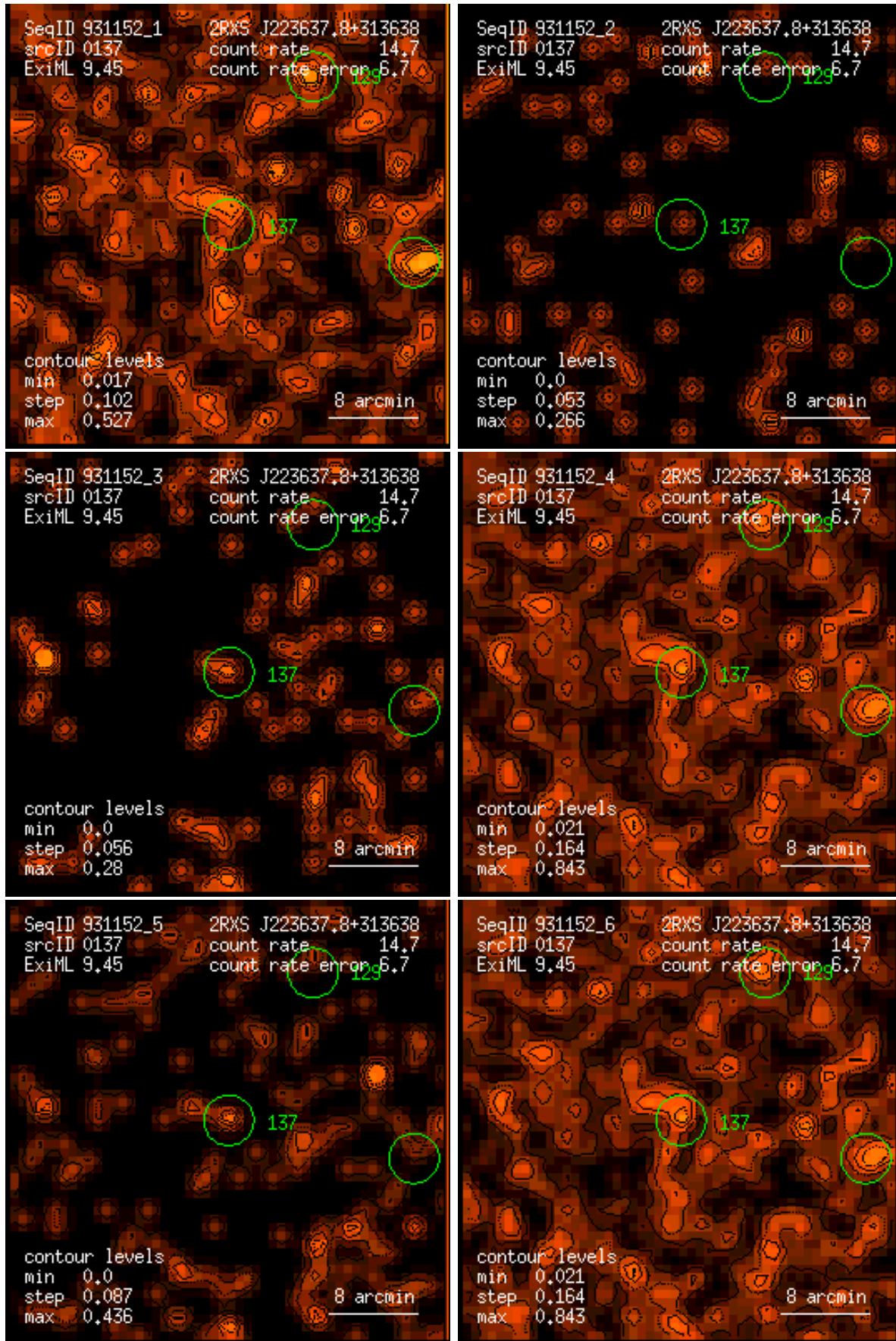
Figure 137: RASS 931152: detection 0137: band rate images, Gaussian filter: (1) PSPC channels 11 – 41, (2) 52 – 90, (3) 91 – 201, (4) 11 – 235, (5) 52 – 201, (6) 11 – 201. Broad band rates in counts/ks. Band rate contour levels in counts/ks/arcmin 2 .
