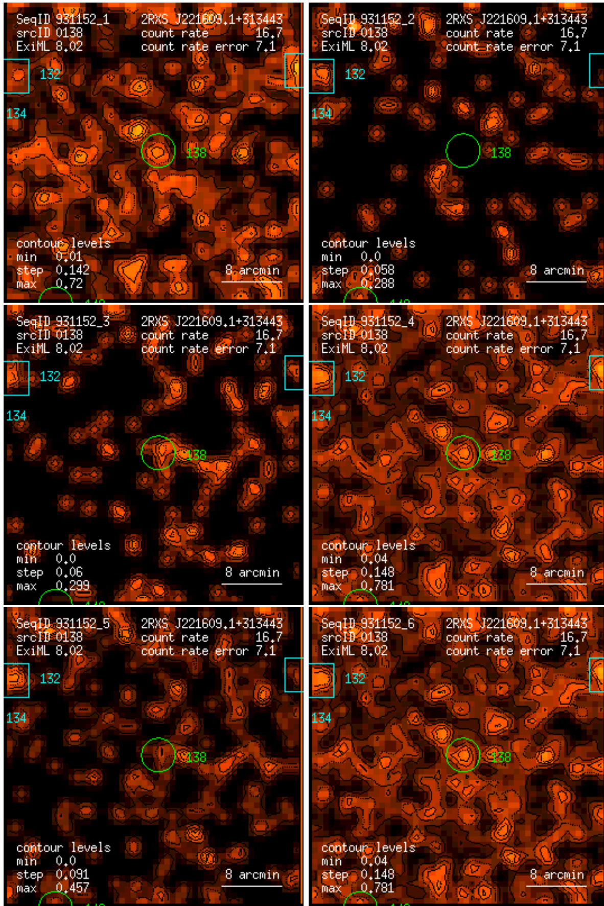
Figure 138: RASS 931152: detection 0138: band rate images, Gaussian filter: (1) PSPC channels 11 – 41, (2) 52 – 90, (3) 91 – 201, (4) 11 – 235, (5) 52 – 201, (6) 11 – 201. Broad band rates in counts/ks. Band rate contour levels in counts/ks/arcmin 2 .
