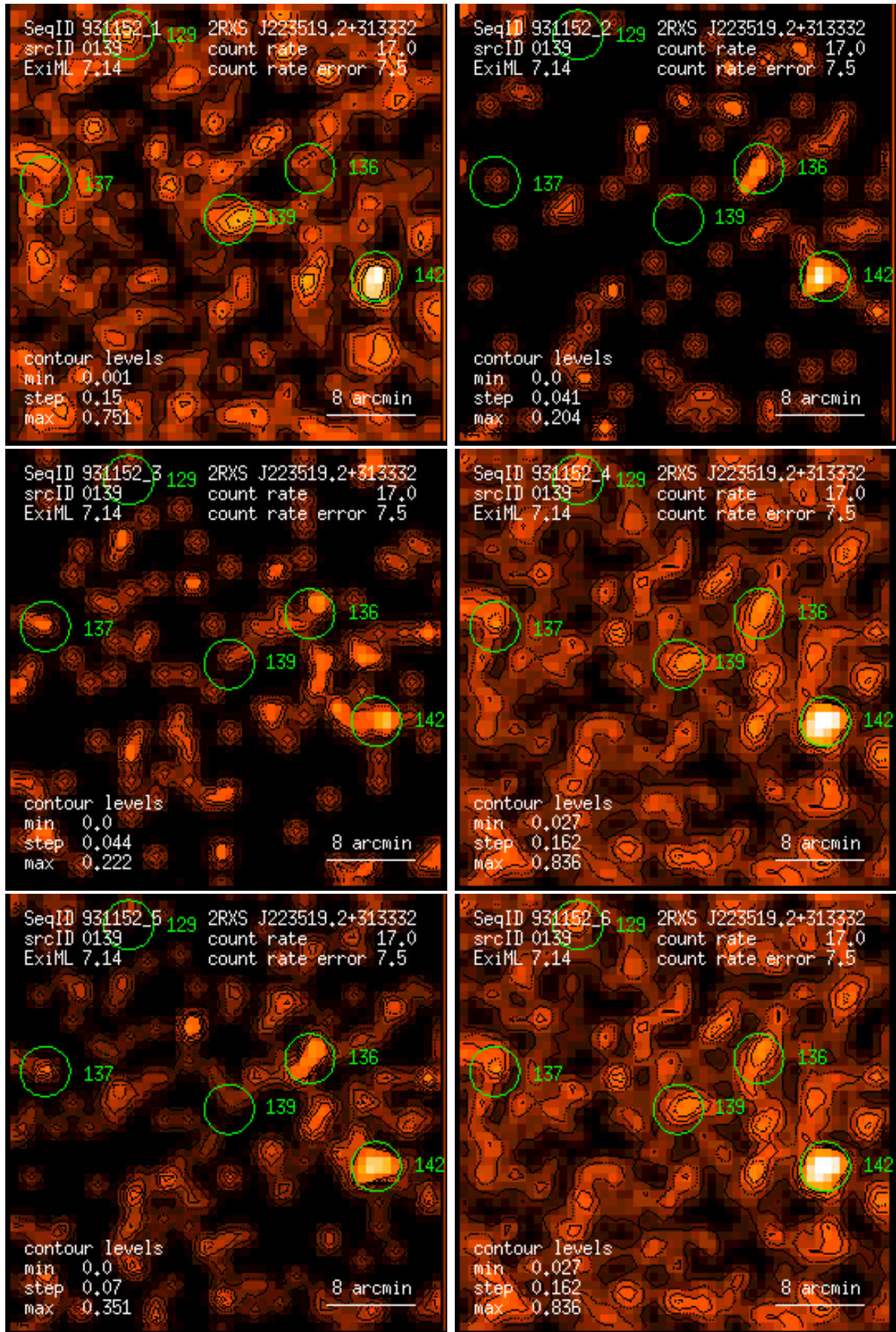
Figure 139: RASS 931152: detection 0139: band rate images, Gaussian filter: (1) PSPC channels 11 – 41, (2) 52 – 90, (3) 91 – 201, (4) 11 – 235, (5) 52 – 201, (6) 11 – 201. Broad band rates in counts/ks. Band rate contour levels in counts/ks/arcmin 2 .
