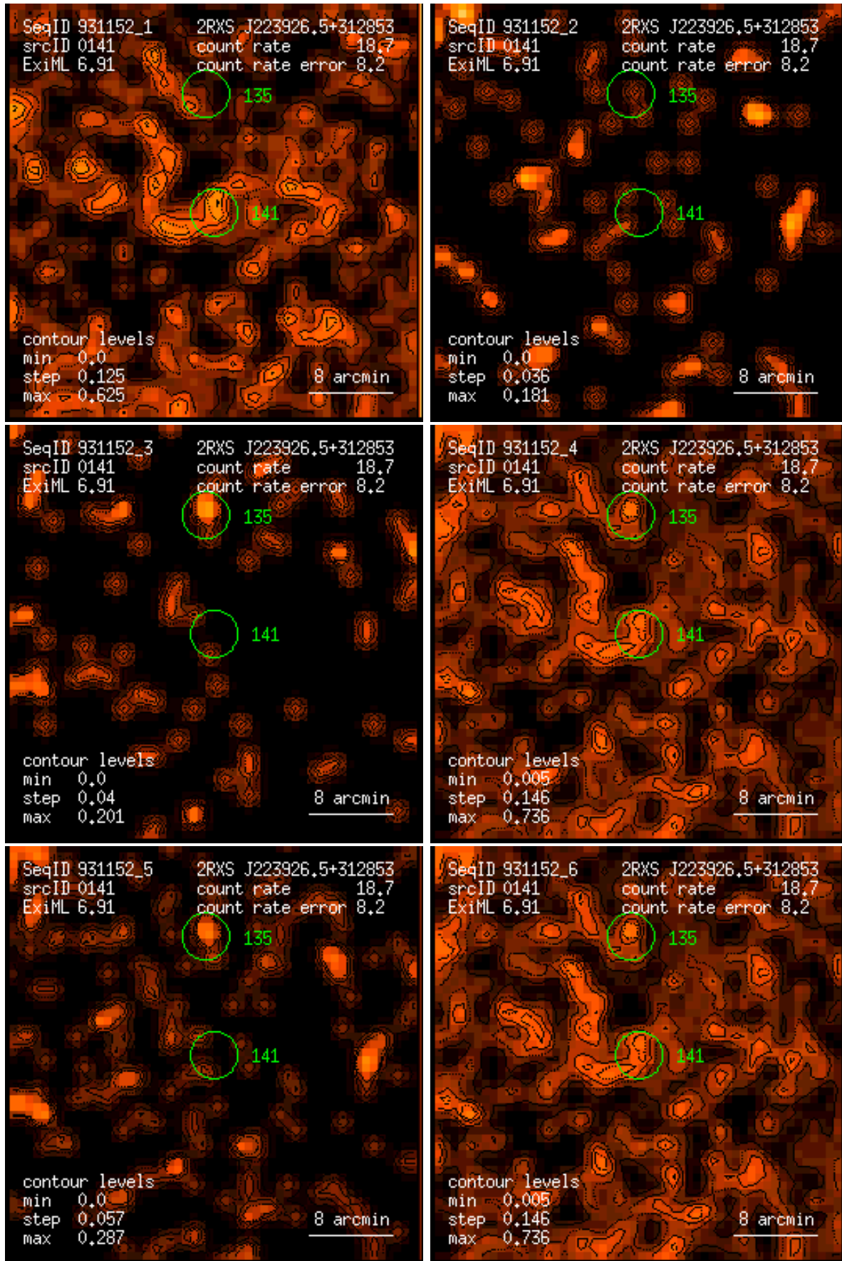
Figure 141: RASS 931152: detection 0141: band rate images, Gaussian filter: (1) PSPC channels 11 – 41, (2) 52 – 90, (3) 91 – 201, (4) 11 – 235, (5) 52 – 201, (6) 11 – 201. Broad band rates in counts/ks. Band rate contour levels in counts/ks/arcmin 2 .
