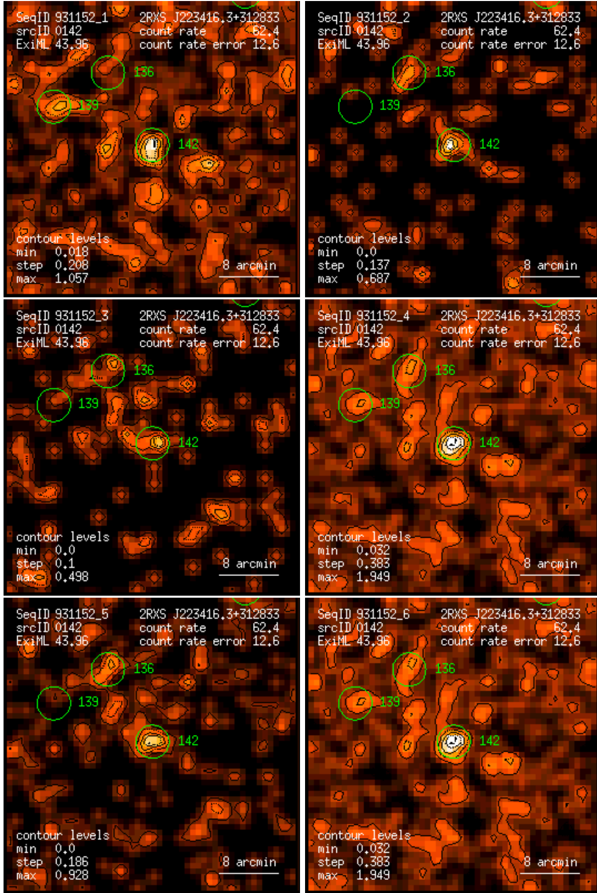
Figure 142: RASS 931152: detection 0142: band rate images, Gaussian filter: (1) PSPC channels 11 – 41, (2) 52 – 90, (3) 91 – 201, (4) 11 – 235, (5) 52 – 201, (6) 11 – 201. Broad band rates in counts/ks. Band rate contour levels in counts/ks/arcmin 2 .
