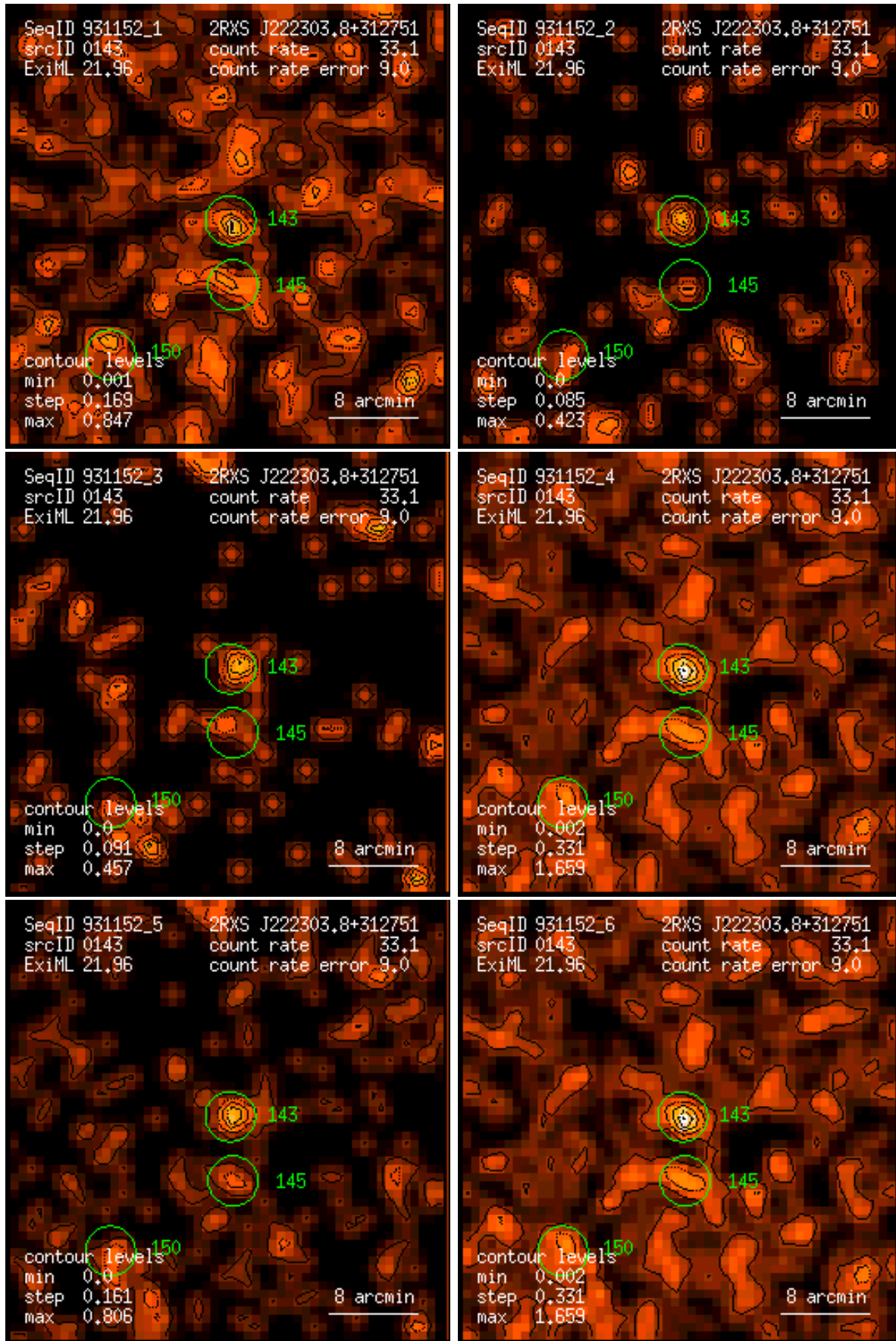
Figure 143: RASS 931152: detection 0143: band rate images, Gaussian filter: (1) PSPC channels 11 – 41, (2) 52 – 90, (3) 91 – 201, (4) 11 – 235, (5) 52 – 201, (6) 11 – 201. Broad band rates in counts/ks. Band rate contour levels in counts/ks/arcmin 2 .
