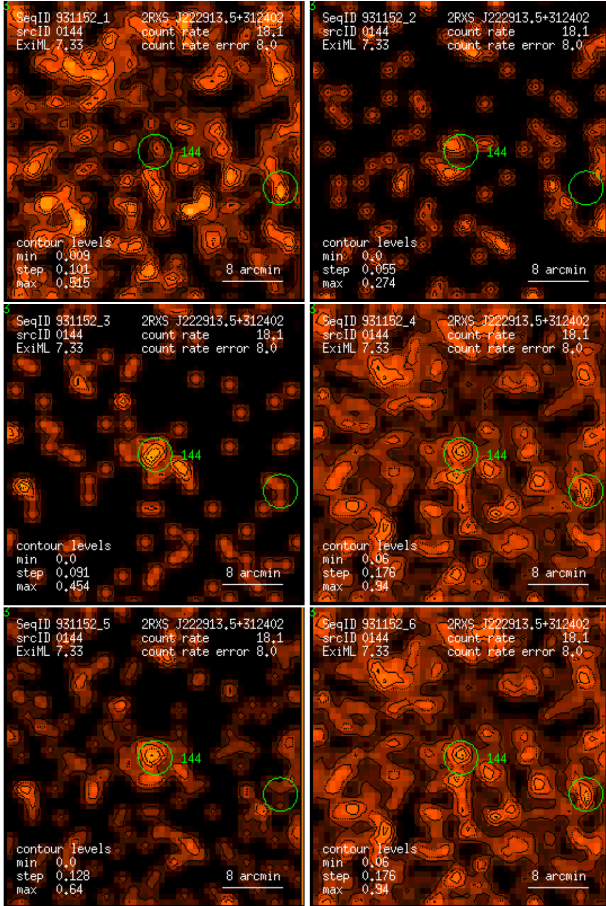
Figure 144: RASS 931152: detection 0144: band rate images, Gaussian filter: (1) PSPC channels 11 – 41, (2) 52 – 90, (3) 91 – 201, (4) 11 – 235, (5) 52 – 201, (6) 11 – 201. Broad band rates in counts/ks. Band rate contour levels in counts/ks/arcmin 2 .
