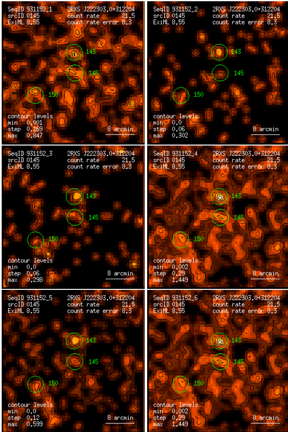
Figure 145: RASS 931152: detection 0145: band rate images, Gaussian filter: (1) PSPC channels 11 – 41, (2) 52 – 90, (3) 91 – 201, (4) 11 – 235, (5) 52 – 201, (6) 11 – 201. Broad band rates in counts/ks. Band rate contour levels in counts/ks/arcmin 2 .
