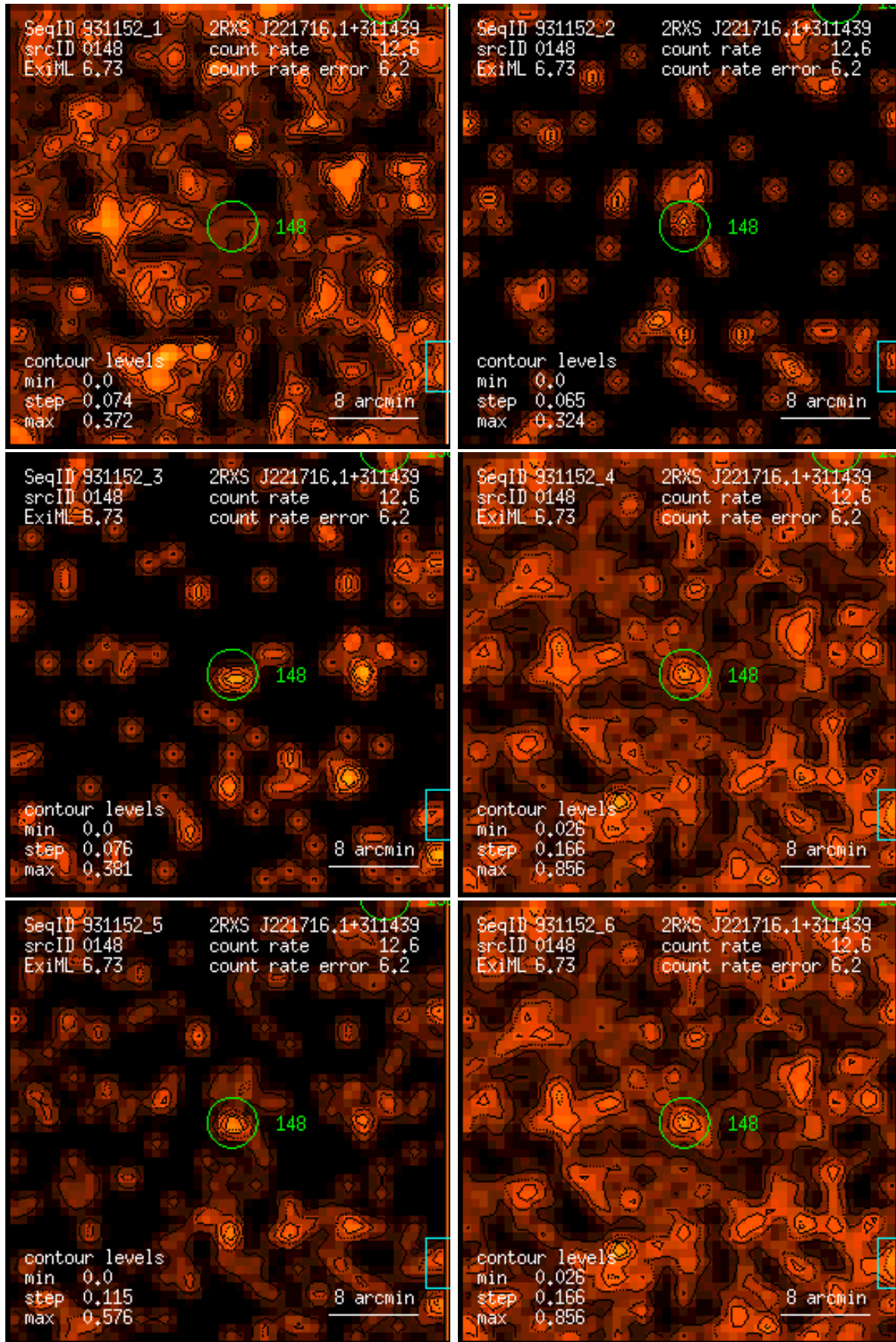
Figure 148: RASS 931152: detection 0148: band rate images, Gaussian filter: (1) PSPC channels 11 – 41, (2) 52 – 90, (3) 91 – 201, (4) 11 – 235, (5) 52 – 201, (6) 11 – 201. Broad band rates in counts/ks. Band rate contour levels in counts/ks/arcmin 2 .
